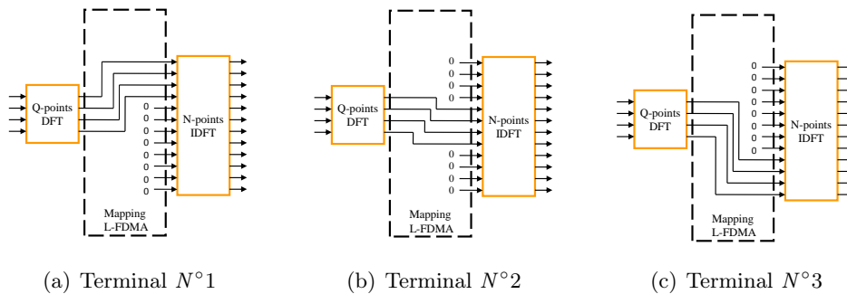
FIGURE 1.11 – Mapping L-FDMA
