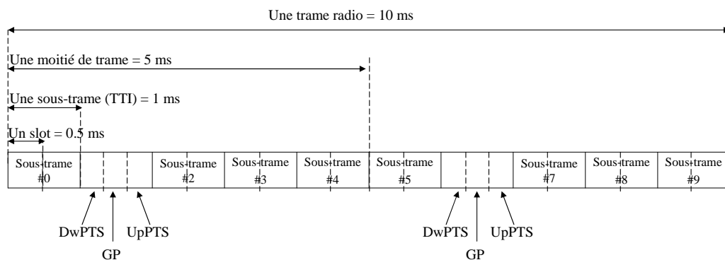
FIGURE 1.24 – Le mode de transmission TDD.
