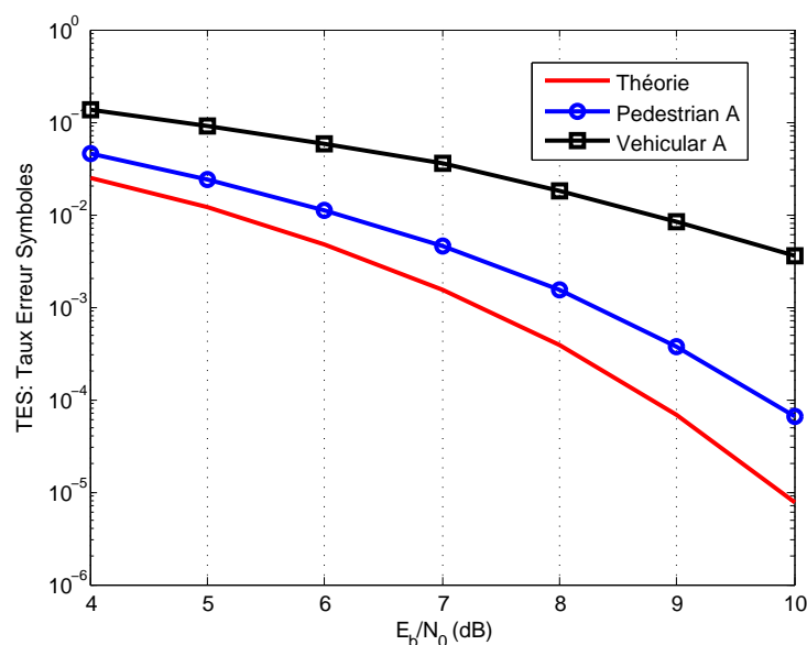
FIGURE 3.1 – Egalisation type ZF : Canal Pedestrian A et Vehicular A
