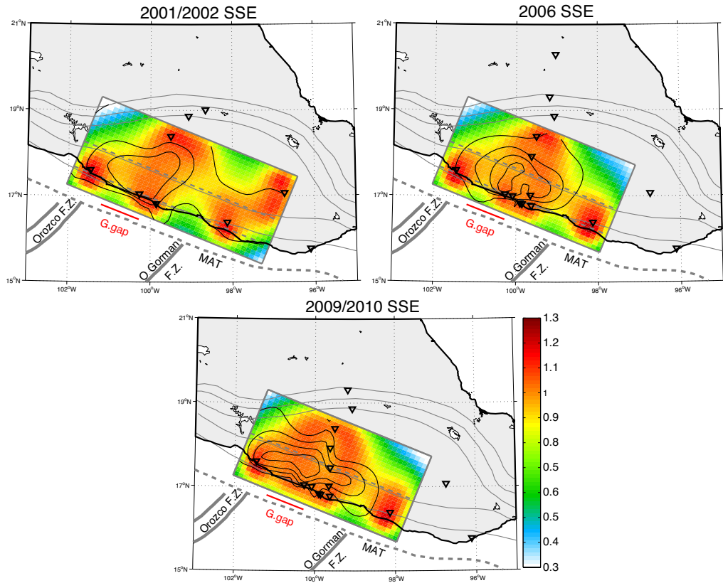
FIGURE 5.13: Resolution map for the inversions of the last three SSEs. The colors represent the value of the restitution index (sum of the lines of the covariance matrix ( Radiguet et al. [2011])). Values close to one represent areas where the slip is well resolved by the inversion. The well resolved areas increased with the increasing number of stations from the 2002 to to 2010. The black contours are the slip contours shown in Figure 4 for each SSE.
