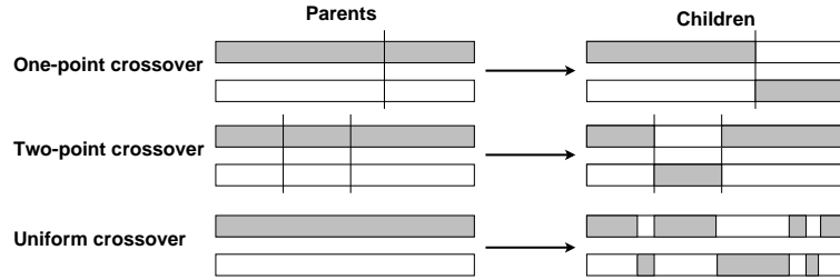
Figure 3.3: Different ways to perform the crossover
