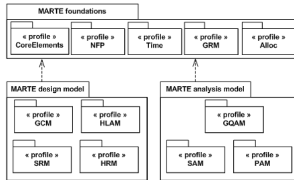
Figure 33. Architecture du profil MARTE [51].
