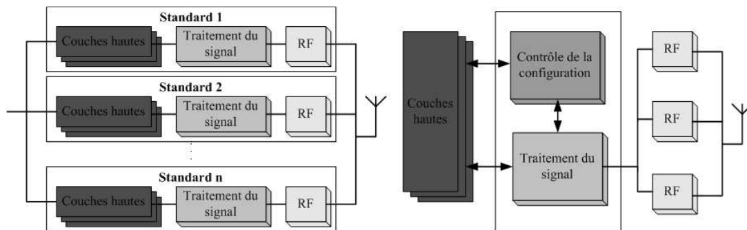
Figure 77. Architecture multistandard classique vs architecture multistandard RLR.
