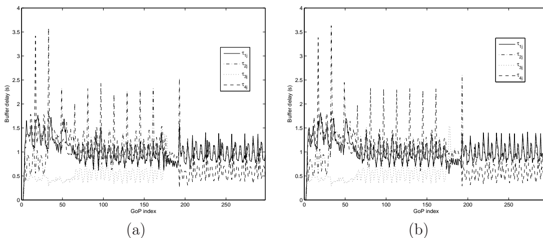
Figure 4.11: Buffer delay evolution of the four multiplexed programs using P, PI, and PID controller with (K_P, K_I, K_D) = (0.4, 0.02, 0.25) for W = 2 (a) and (K_P, K_I, K_D) = (0.5, 0.02, 0.25) for W = 4 (b) with constant channel rate, when buffers bit levels are controlled.
