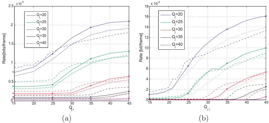
Figure 3.3: Rate as a function of Q_{j-1} , parameterized with Q_j ; compound model (dashed), total rate using H.264/AVC (solid), texture rate using H.264/AVC (dotted) for Soccer(a) and Container(b) sequences.
