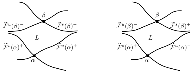
(a) A lozenge of type (+, +, -, -) (b) A lozenge of type (+, -, -, +)
