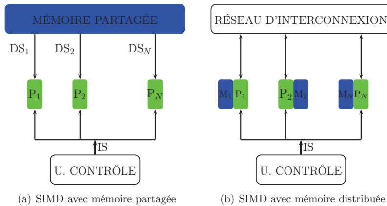
FIGURE 1.3 – Architecture SIMD (Single Instruction Multiple Data)
