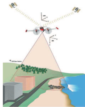
FIGURE 1.1 – Lidar scanner
