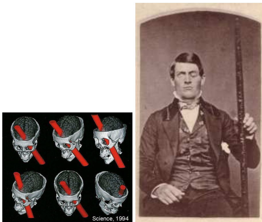
Fig. 1-4 – Phineas Gage.
