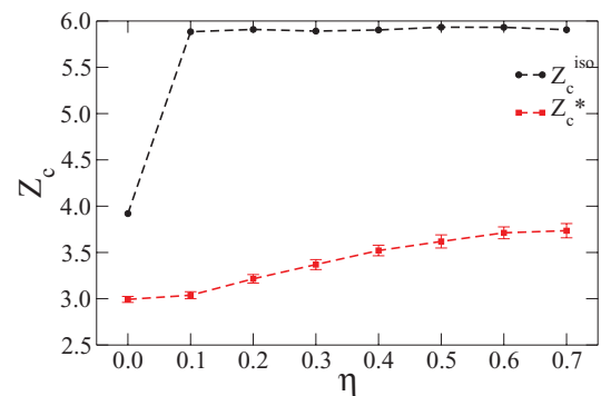
FIG. 9. (Color online) Connectivity number Z_c in the initial isotropic state (labeled by “iso”) and in the residual state (labeled by \star ) as a function of nonconvexity \eta . The error bars of Z_c^* indicate the standard deviation of the data in the residual state.
