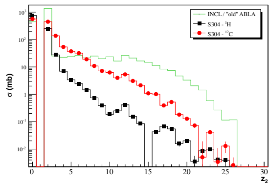
FIGURE 4.49 – \sigma(z_2) (mb).
