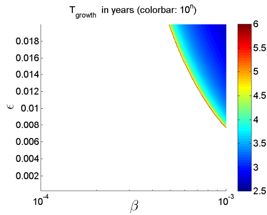
FIGURE 4.17 – Same as figure 4.16 but for Europa, considering (a) its possible liquid core and (b) a 100 km depth subsurface ocean. Both the core and the subsurface ocean of Europa are expected to behave in the deformable limit, locating their states in the upper right corner of the diagram. Both are thus found to be unstable.
