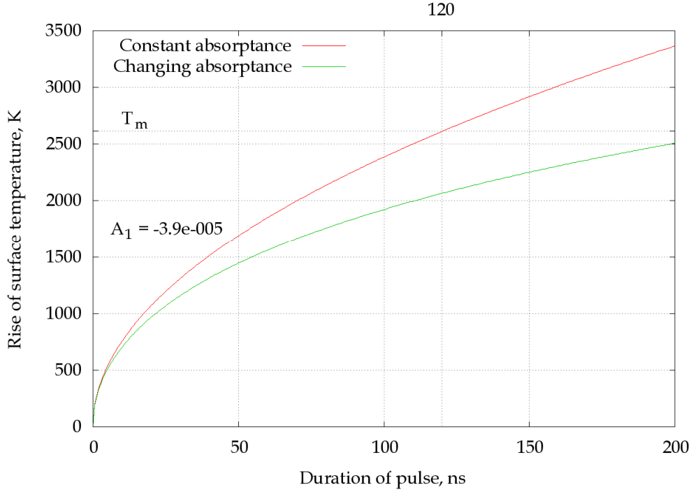
Figure 14: Time dependence of molybdenum surface temperature.
