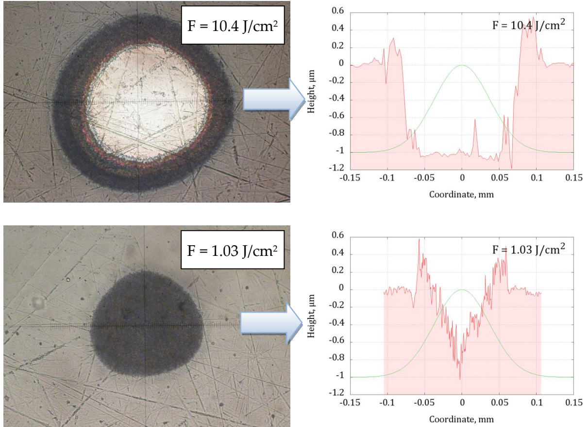
Figure 58: Photos and 1D profiles of craters formed on the surface of W/W+αCH sample under the action of laser pulses with fluence F = 10.4 \text{ J/cm}^2 and F = 1.03 \text{ J/cm}^2
