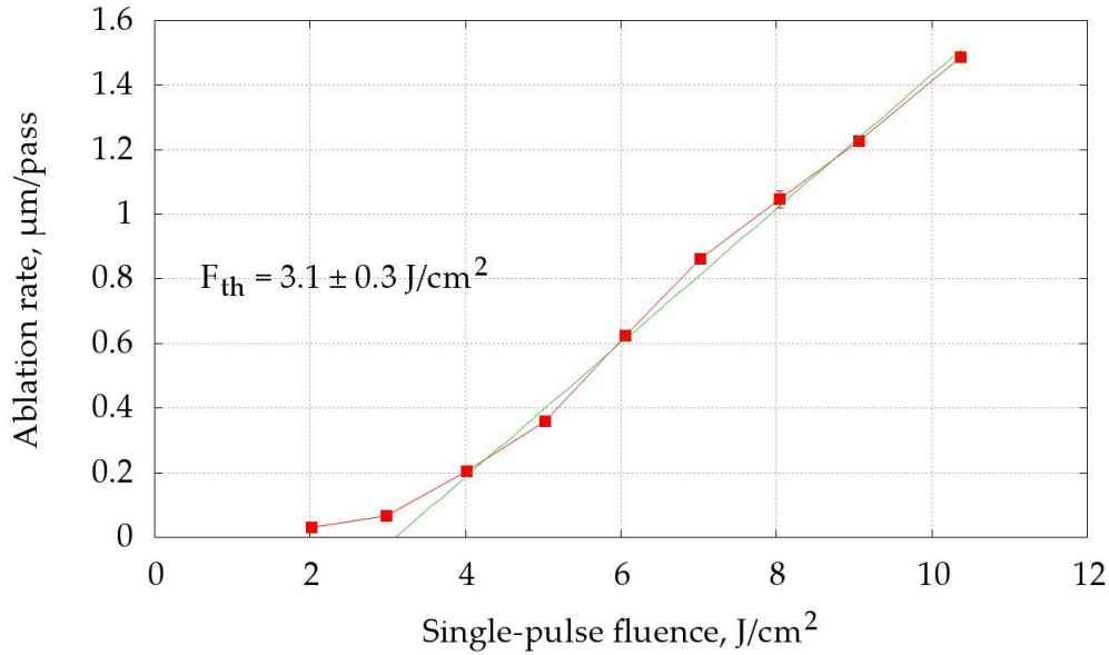
Figure 41: Dependence of the oxide layer ablation rate on the laser fluence. Sample was oxidized in furnace. Oxide layer thickness is 5 - 6 \text{ } \mu\text{m} .
