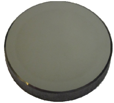
Round Mo mirror Diameter d = 25\text{ mm} Thickness h = 4.7\text{ mm}
