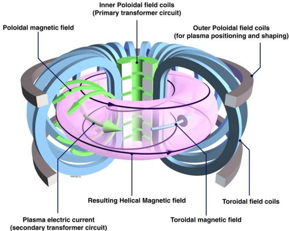
Figure 5: Scheme of a tokamak.
