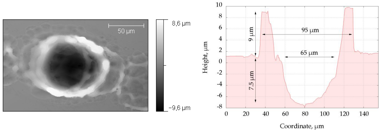
Figure 70: Profile of a crater on the surface of the SS mirror after application of ~5000 shots with E=0.93 \text{ mJ} , F=10.54 \text{ J/cm}^2
