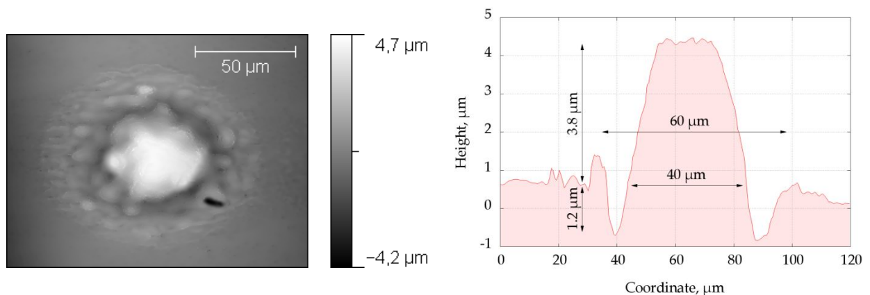
Figure 71: Profile of a crater on the surface of the Mo mirror after application of ~5000 shots with E=0.93 \text{ mJ} , F=10.54 \text{ J/cm}^2
