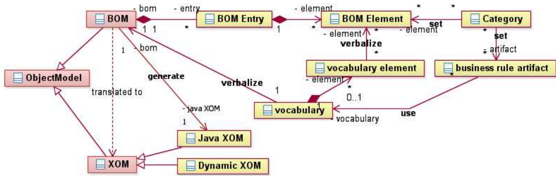
Figure A-3. Relationships between BOM and XOM in JRules
