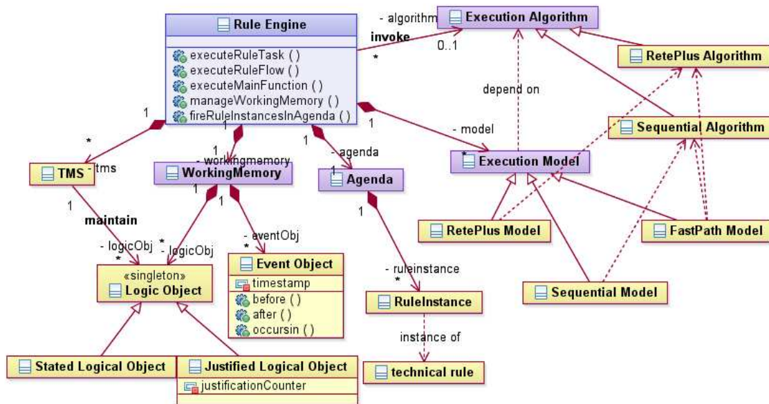
Figure A-9. Concepts in the Rule Engine of JRules
