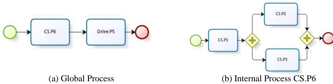
Figure 3-10. Simplified Cooperation Process for ShoppingDrive
