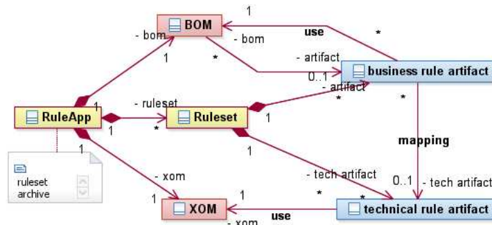
Figure A-6. Ruleset Archive in JRules
