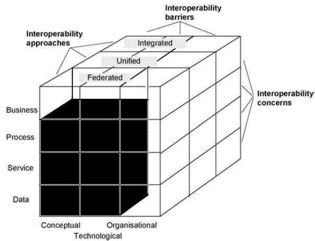
(c) Enterprise Interoperability Framework (with three dimensions) from INTEROP (Chen and Daclin 2006; Chen, Doumeingts et al. 2008)
