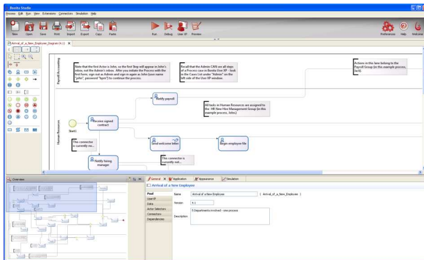
Figure C-10. Bonita Studio
