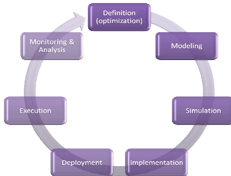
Figure 2-2. BPM lifecycle
