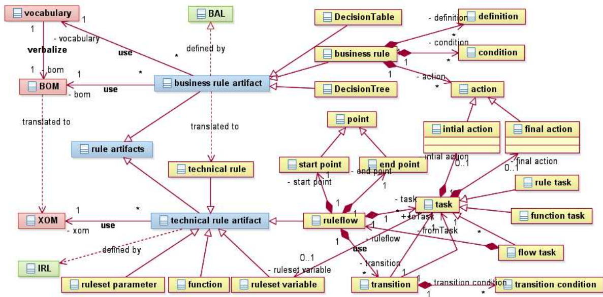
Figure A-5. Relationships between Business and Technical Rule Artifacts in JRules
