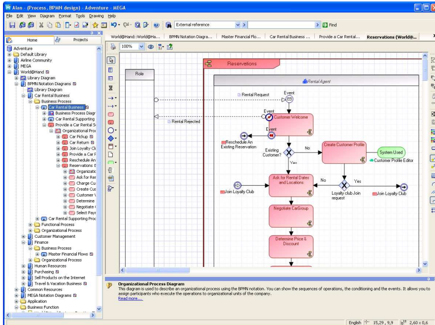
Figure C-18. MEGA
