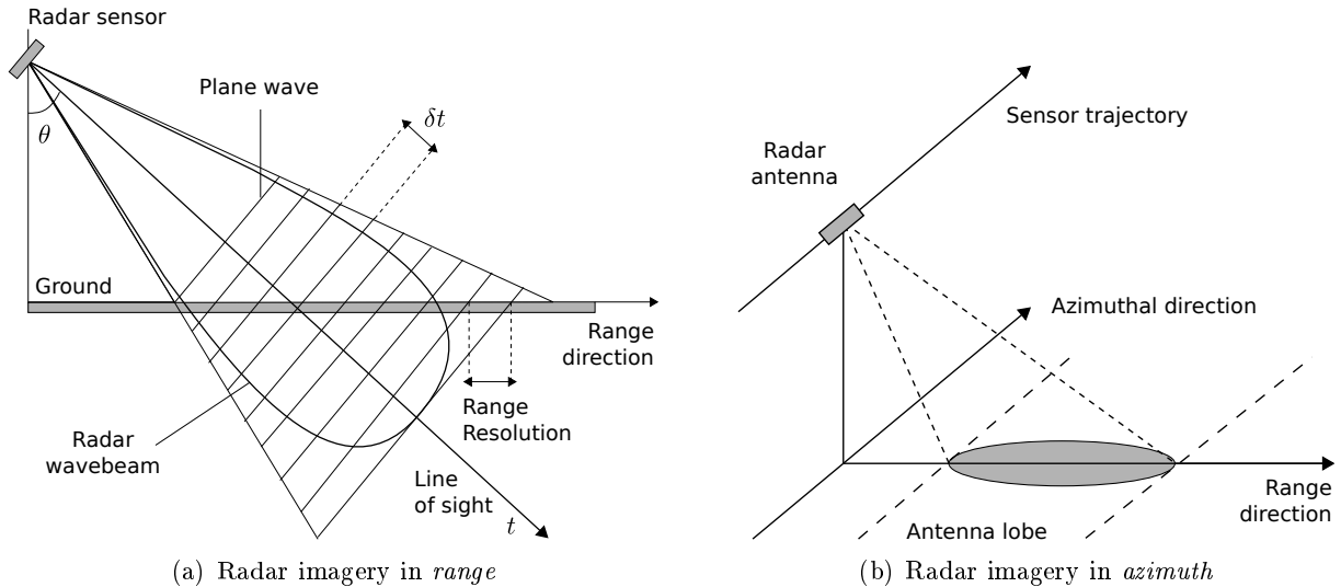
Figure 6.1: (a) Principle of line construction in a radar image. Thanks to the use of a non-null incidence angle \theta , objects located at different positions on the ground in the range direction will be projected at different positions on the line of sight. (b) Principle of column construction in a radar image. The radar sensor acquires the different lines by moving in the azimuthal direction.
