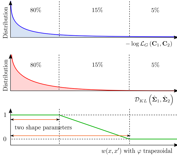
Figure 6.14: (top) Distribution of GLR when the two compared noisy patches share a common noise-free patch. (center) Distribution of the symmetrical Kullback-Leibler divergence when the two compared pre-filtered patches share a common noise-free patch. (bottom) According to this probability of false alarm, we can define the shape of a trapezoidal kernel function to control the amount of smoothing.
