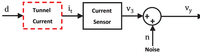
Figure 3.3: Block diagram representation of tunneling current and current sensor (dashed block indicates the nonlinear element).
