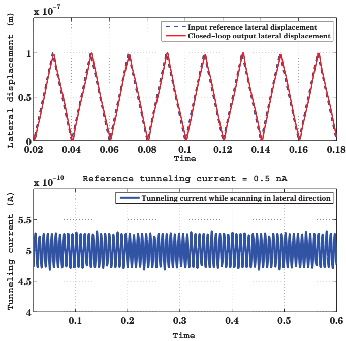
Figure 5.14: With MIMO control, the horizontal scanning speed of 100 \text{ Hz} with scanning range of 0.1 \mu\text{m} and corresponding tunneling current variations in vertical z -direction in the presence of sinusoidal surface variations ( z_S ) of frequency of 800 \text{ rad/sec} ( 127.32 \text{ Hz} ) and an amplitude of 0.5 \text{ \AA} .
