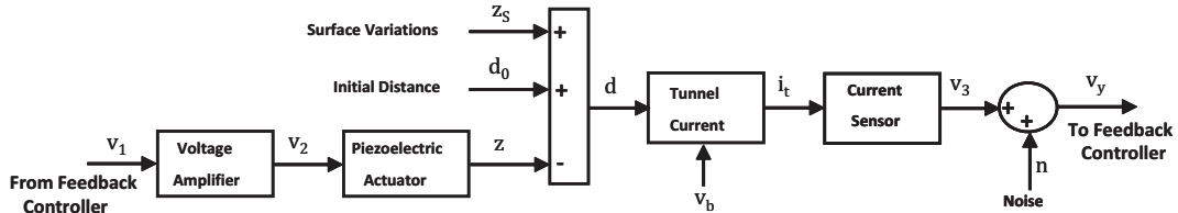
Figure 3.2: Open loop system with block diagram representation.
