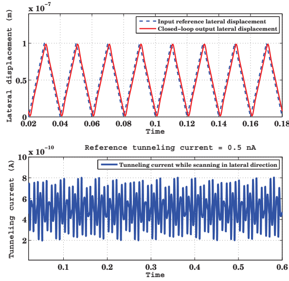
Figure 5.12: Simulation result with horizontal scanning speed of 100 \text{ Hz} , scanning range of 0.1 \text{ } \mu\text{m} and corresponding tunneling current variations in vertical z -direction in the presence of sinusoidal surface variations ( z_s ) of frequency of 800 \text{ rad/sec} ( 127.32 \text{ Hz} ) and an amplitude of 0.5 \text{ } \text{\AA} .
