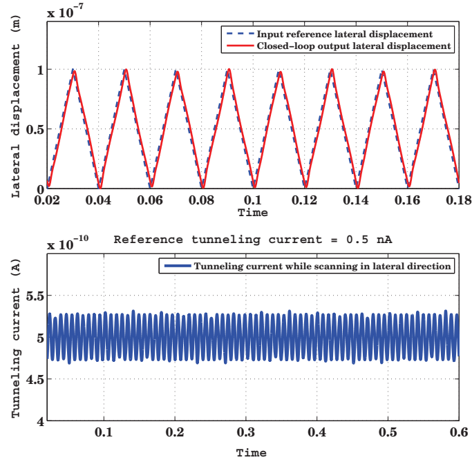
Figure 5.14: With MIMO control, the horizontal scanning speed of 100\text{ Hz} with scanning range of 0.1\text{ }\mu\text{m} and corresponding tunneling current variations in vertical z -direction in the presence of sinusoidal surface variations ( z_S ) of frequency of 800\text{ rad/sec} ( 127.32\text{ Hz} ) and an amplitude of 0.5\text{ \AA} .
