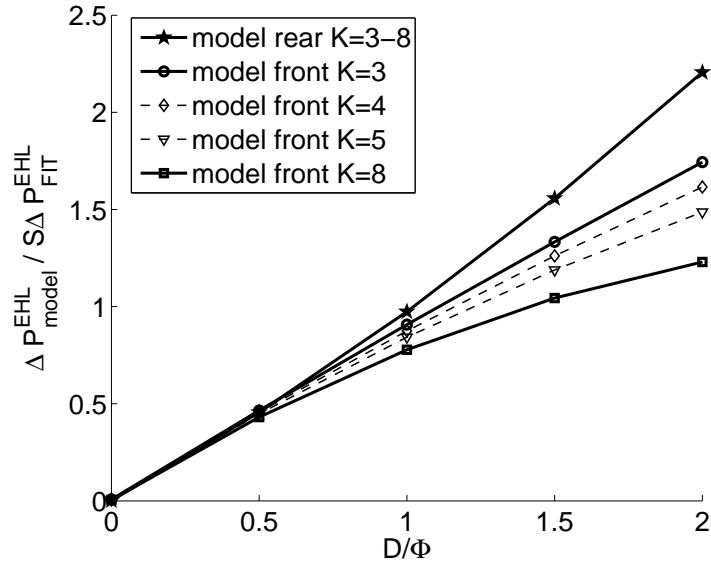
Figure 3.25: \Delta P_{FRONT}^{EHL}/S\Delta P_{FRONTFIT}^{EHL} and \Delta P_{REAR}^{EHL}/S\Delta P_{REARFIT}^{EHL} for deeper indents. M = 100 - 1200 , L = 3 - 19 , \Phi = 0.25 - 1 and K = 3 - 8
