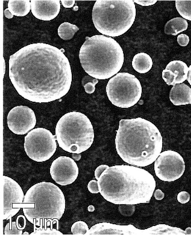
Figure 1.4: M50 particles [119] (distribution 0 – 100 \mu m )
