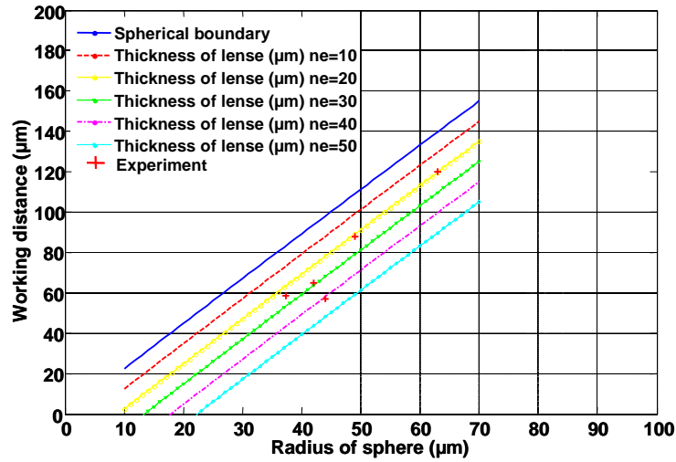
Fig 12. Working distance versus radius of osculating sphere of a Gradhyp for several effective thickness n_e .
