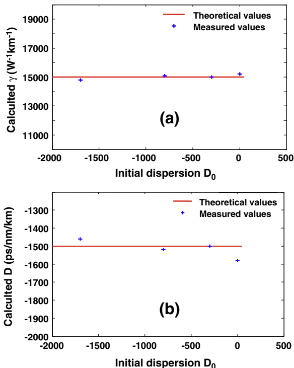
Fig. 5. Calculated results of the nonlinear coefficient and the dispersion for different initial values D_0 .
