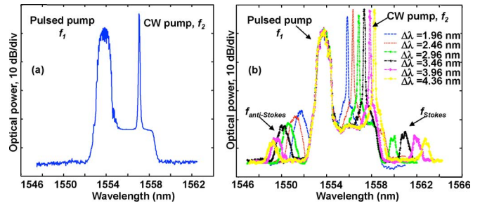
Fig. 4. (a) Input spectra of CW and pulsed pumps and (b) output spectra of the chalcogenide fiber.
