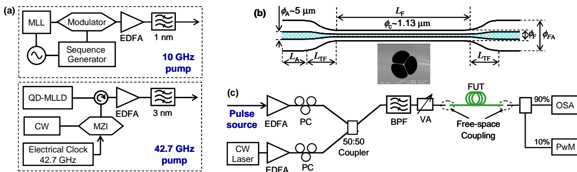
Fig. 1: (a) Block diagram of pulses stream generation for (top) 10\text{ GHz} and (bottom) 42.7\text{ GHz} signal; (b) Suspended-core chalcogenide fiber with mode adaptation ends; and (c) Setup of FWM measurement.
