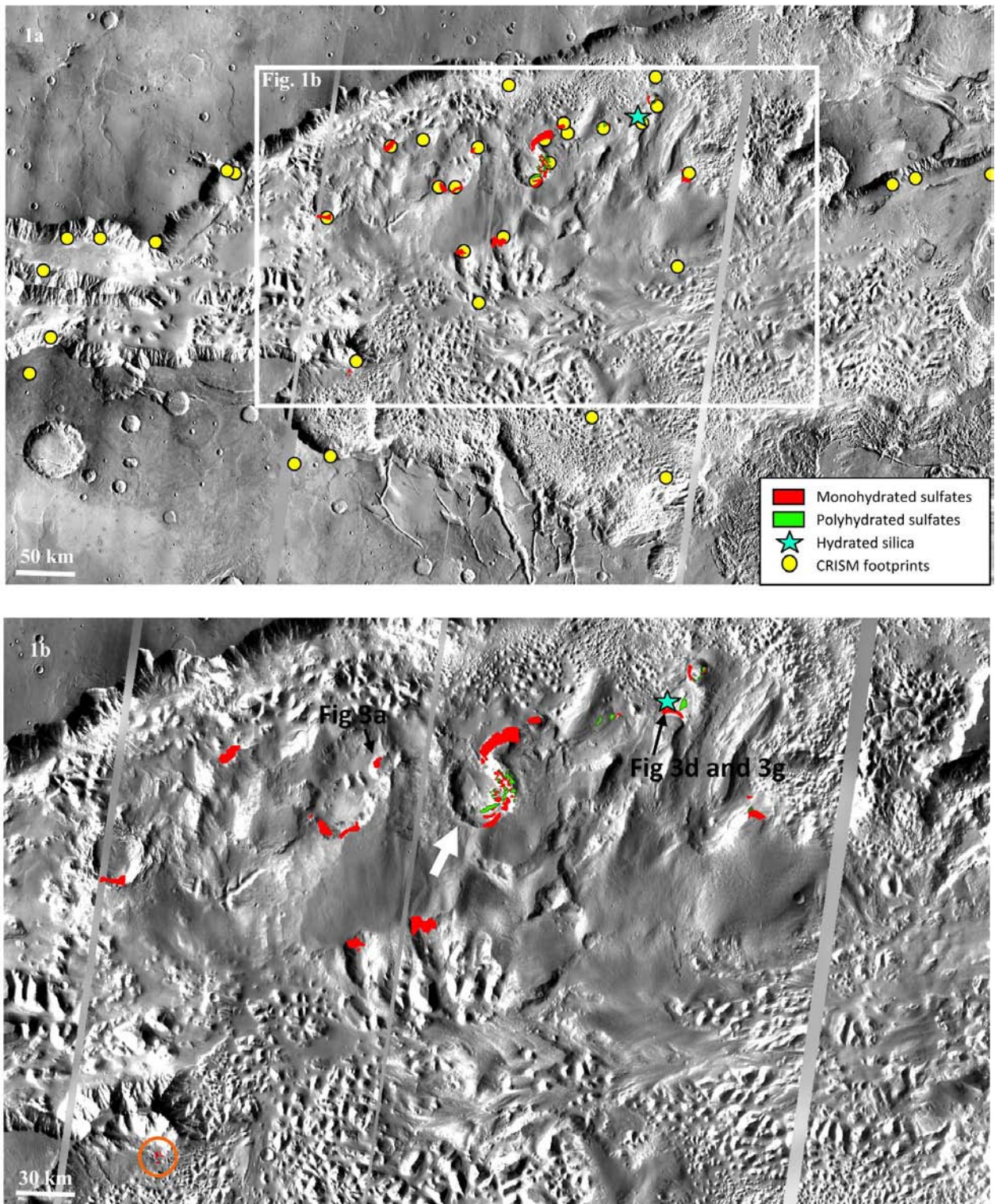
Figure 5.15: (a) Distribution of the main hydrated mineral detections in Capri Chasma (central longitude: 46.5^{\circ}\text{E} , central latitude: 14.5^{\circ}\text{S} ). The white box indicates the location of Figure 5.15b. Yellow dots, CRISM footprints; red, monohydrated sulfates; green, polyhydrated sulfates; blue star, opaline silica, detected in a smaller amount. (b) Close-up on the main mesa of the ILD, showing sulfate detections above the flanks.
