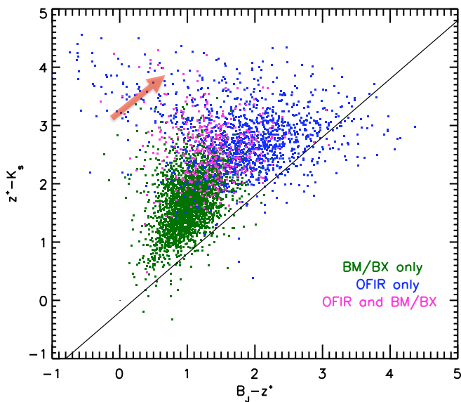
Fig. 4. Distribution of the 24\mu\text{m} sources selected as optically-faint IR-bright galaxies (blue dots) and with the BM/BX criterion (green dots) in the BzK diagram. Only sources at 1.5 < z < 2.8 are represented and galaxies satisfying the two selections are shown with pink color. The Optically-Faint IR-bright sources are characterized by redder colors, most likely due to higher dust extinction. The red arrow represents the extinction vector.
