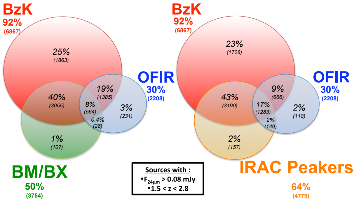
Fig. 5. Overlap between the populations of 24\mu\text{m} sources with F_{24\mu\text{m}} > 0.08 mJy on the redshift range 1.5 < z < 2.8 . The percentages in bold are related to the total number of sources selected by the criterion considered, the percentages in italic correspond to the overlap between the populations. Left: Overlap between the BzK, the BM/BX and the Optically Faint IR-bright sources. Right: Overlap between the BzK, the Optically Faint IR-bright sources and the IRAC Peakers.
