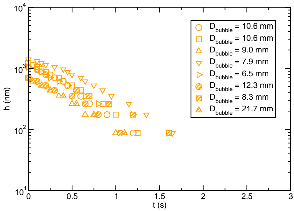
Figure G.17: Evolution of thickness for various bubble size in soda-lime-silica glass with 0.1 wt% of Fe_2O_3 and temperature 1228^\circ C .
