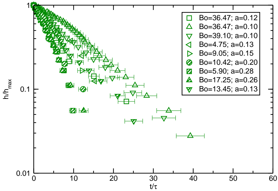
Figure G.16: Normalized evolution of thickness for various bubble size in soda-lime-silica glass with 0.1 wt% of Fe_2O_3 and temperature 1142^\circ C .
