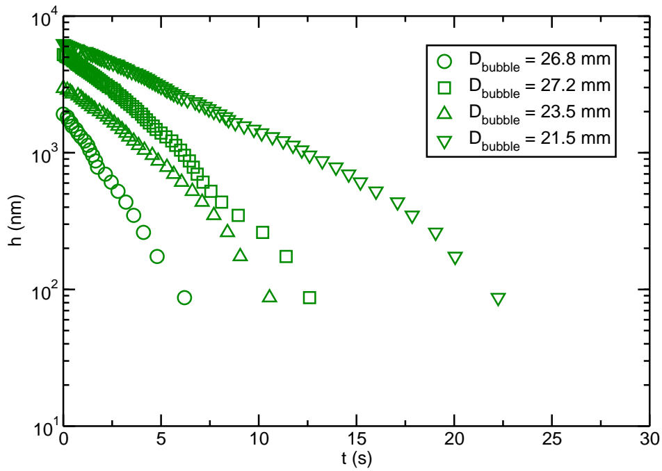
Figure G.19: Evolution of thickness for various bubble size in soda-lime-silica glass with 1 wt% of B_2O_3 and temperature 1142^\circ C .
