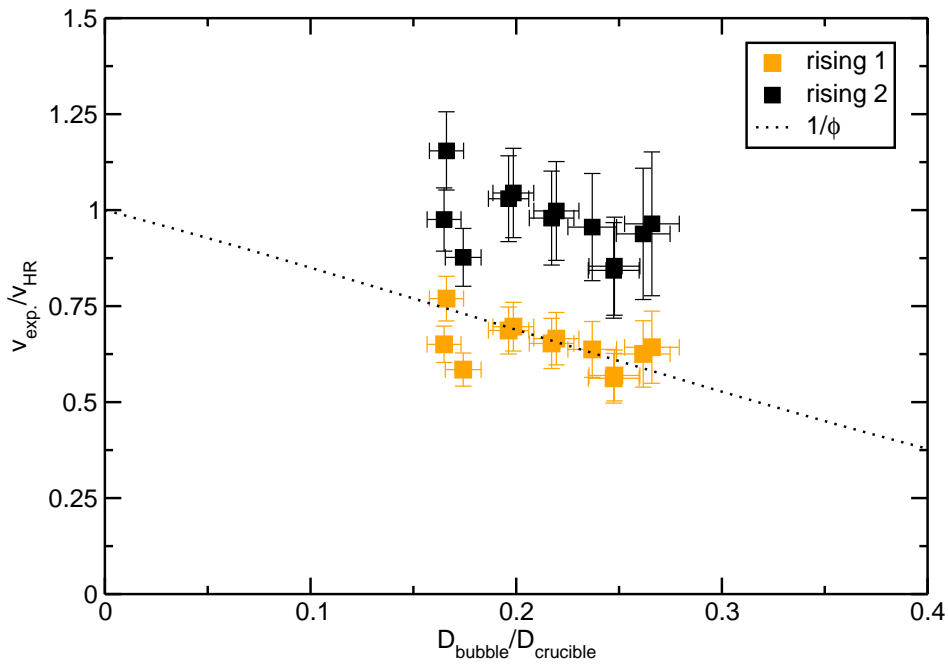
Figure 6.3: Comparison of two experimental rising velocities in glass with 0.1 wt% of Fe_2O_3 at T_E=1228^\circ C .
