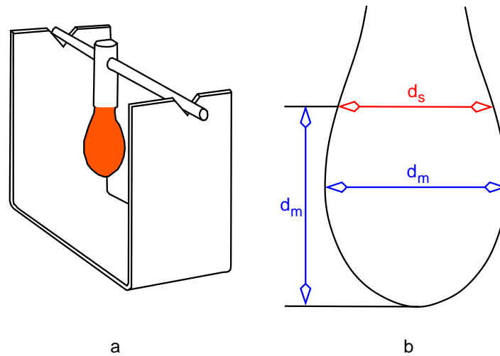
Figure 2.5: Determination of surface tension: pendant-drop method [19].
