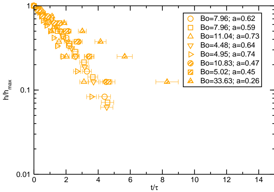
Figure G.18: Normalized evolution of thickness for various bubble size in soda-lime-silica glass with 0.1 wt% of Fe_2O_3 and temperature 1228^\circ C .
