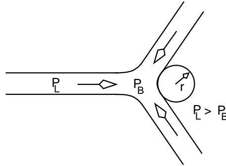
Figure 3.3: Plateau border suction.
