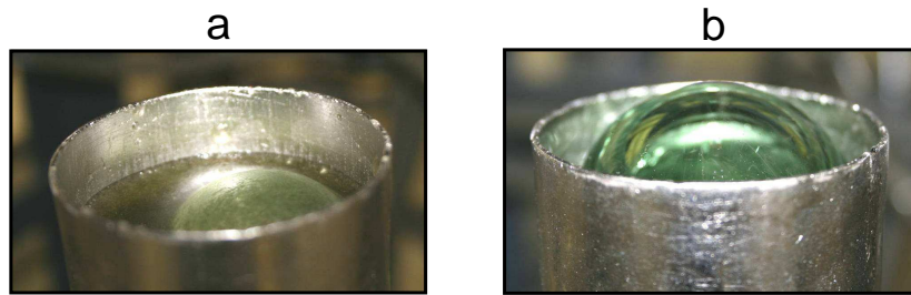
Figure 5.5: Captured bubble in glass with 1 wt% \text{Fe}_2\text{O}_3 with crystals on the surface (a) and without (b).
