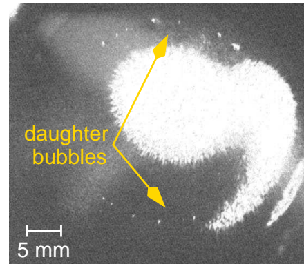
Figure 6.68: Ring of daughter bubbles.
