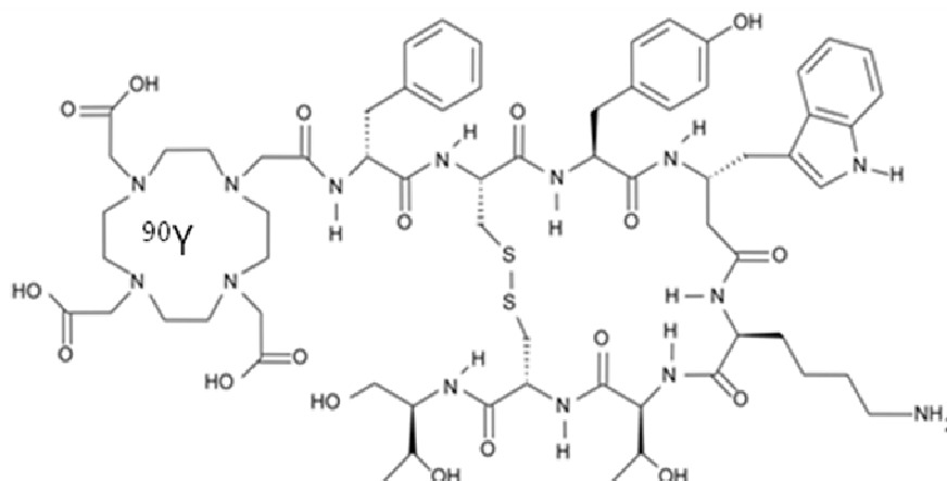
Figure 3: Structure of 90 Y-DOTATOC
