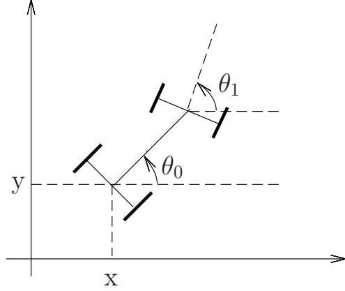
Figure 1.1: nonholonomic car
