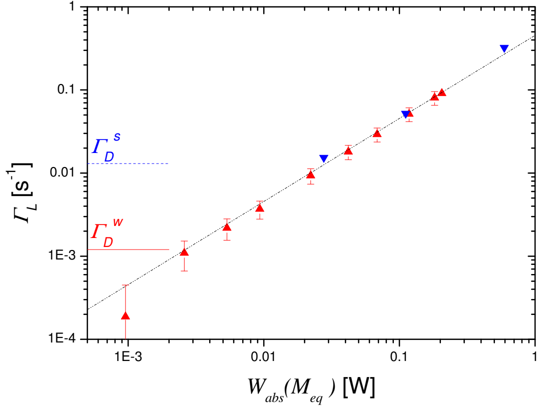
Figure 6.53: Difference between total relaxation rate \Gamma_R and decay rate \Gamma_D ( \Gamma_R - \Gamma_D = \Gamma_L ) at steady state polarisation M_{\text{eq}} at p_3 = 2.45 mbar, B = 1 mT and OP on \text{C}_8 as function of absorbed laser power. (Red) triangles: weak discharge (parameters see caption of figure 6.50), (blue) downward triangles: strong discharge, n_m^S(M = 0) = 4.15 \times 10^{16} \text{ atoms/m}^3 , \Gamma_D^s = 0.013 \text{ s}^{-1} . Dash-dotted line: guide for the eye ( y = x/2.2 ) from figure 6.50. Errors in x-direction on W_{\text{abs}}(M_{\text{eq}}) are smaller than at 0.63 mbar due to higher SNR of the pump transmission coefficient at 2.45 mbar.
