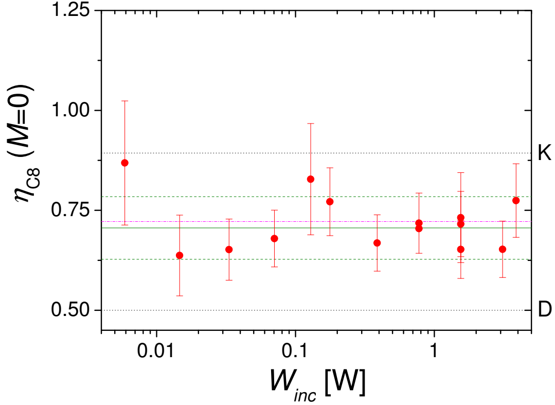
Figure 6.43: Photon efficiency of C_8 pump transition at p_3 = 2.45 mbar as function of incident pump laser power: Compilation of \eta_{C8}(M = 0) = \eta_{C8}(M) of various experiments. (Green) Solid line: weighted mean value of experimental data points: 0.706. (Green) Dashed lines: weighted mean value \pm standard deviation \sigma_\eta : 0.084. Other lines: see caption of figure 6.41. Errors will be reviewed in the final published version of data.
