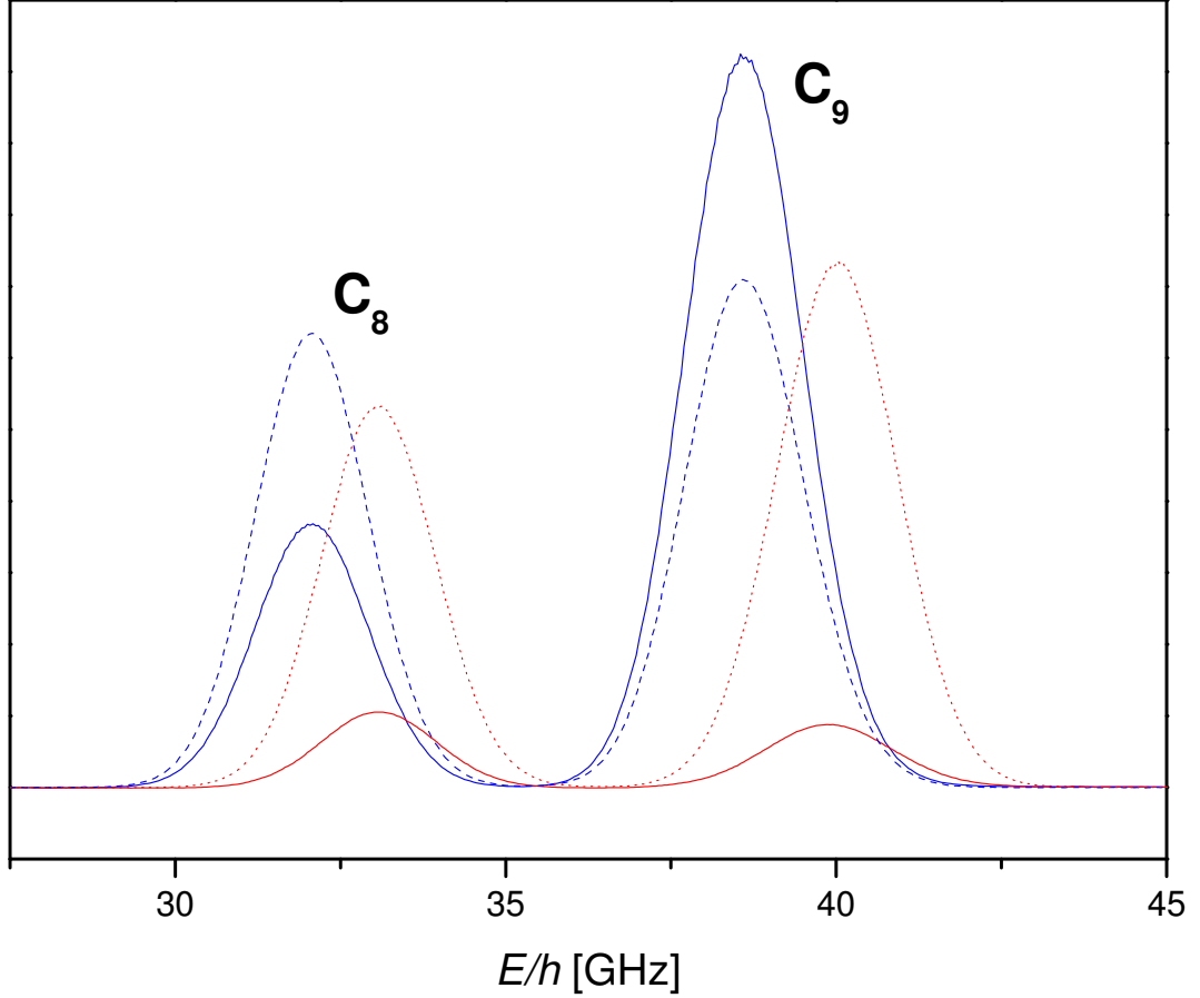
Figure 4.3: Experimental absorption spectrum of ^3\text{He} at B = 30 mT, p_3 = 1.07 mbar: Intensity (same convention as in figure 4.2) as function of probe laser frequency for M = 0 (dashed line: \sigma^- , dotted line: \sigma^+ ) and M = 0.5 (solid lines for both \sigma^- and \sigma^+ , distinguishable by peak positions: same as at M = 0 ). This sweep of the probe laser frequency is recorded during a polarisation decay: the pump laser is turned off and the decay rate of \Gamma_D = (238 \text{ s})^{-1} is sufficiently low so that M = \text{constant} during a complete frequency sweep from approximately 27.5 GHz to 45 GHz within 10 to 20 s typically (frequency swept at 0.05-0.1 Hz approximately, leading to a sweeping rate of roughly 0.9-1.8 GHz/s).
