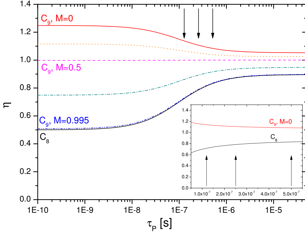
Figure 2.15: Computed photon efficiencies (parameters used for computations: see caption of figure 2.14) for C_8 and C_9 as function of the intrinsic relaxation time in the 2^3\text{P} state for different M values. Lines from top to bottom: solid: C_9, M = 0 ; dot: C_9, M = 0.3 ; dash: C_9, M = 0.5 ; dash-dot: C_9, M = 0.8 ; dash-dot-dot: C_9, M = 0.995 ; solid: C_8 (independent of M ). Inset: \eta as function of \tau_P in seconds (linear scale). Top: C_9, M = 0 ; bottom: C_8 . The arrows in main plot and inset indicate the empirically determined values of \tau_P (see chapter 6.3.2) for the different values of ^3\text{He} pressure. From left to right: 2.45 mbar, 1.19 mbar and 0.63 mbar. B = 1 mT.
