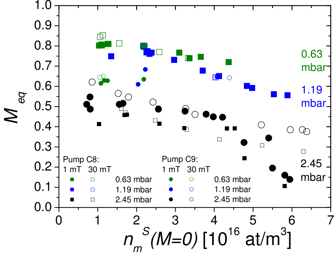
Figure 6.57: Steady state polarisation as function of metastable density n_m^S(M=0) at fixed W_{\text{inc}} = 1.66 W at B = 1 mT (filled symbols) and B = 30 mT (open symbols). Squares: C 8 pump transition, circles: C 9 pump transition. Three values of ^3\text{He} pressure: Green symbols: 0.63 mbar, blue symbols: 1.19 mbar, black symbols: 2.45 mbar. For each pressure, data of the respective pumping line yielding highest M_{\text{eq}} values are represented by big symbols.
