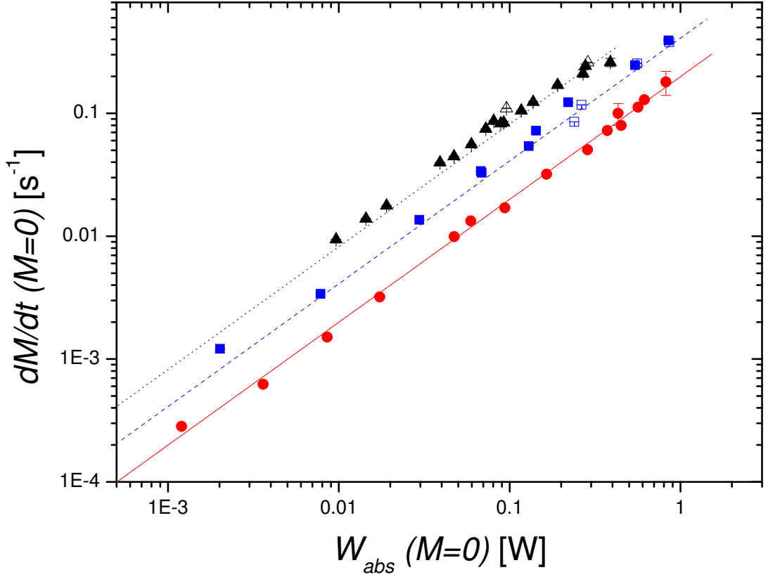
Figure 6.40: Experimental and computed values of \dot{M}(0) (symbols and lines respectively) as function of absorbed laser power (comprising data of several different discharges), both on the \text{C}_8 -pump-transition at M = 0 for three different pressure values: 0.63 mbar (triangles and dotted line), 1.19 mbar (squares and dashed line), and 2.45 mbar (circles and solid line). Filled symbols: probe \text{C}_8 , open symbols: probe \text{C}_9 . Whenever experimental error bars are invisible, they are smaller than the size of the symbols. Computations use empirically determined values of \gamma_r^{\text{P}} (see subsection 6.3.2).
