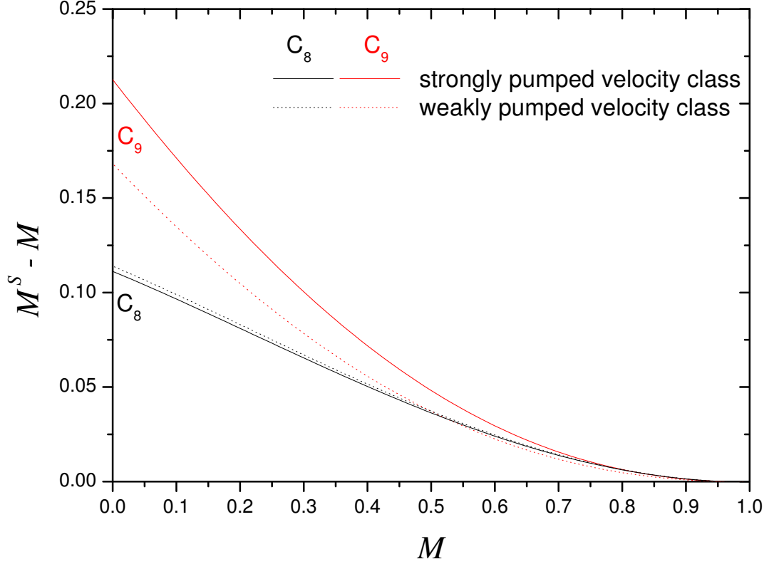
Figure 2.13: Computed difference between 2^3\text{S} polarisation M^S and ground state polarisation M under influence of OP on \text{C}_8 (black) and \text{C}_9 (red) transitions with W_{\text{inc}} = 1 \text{ W} , \sigma^+ light, for the strongly (straight lines) and weakly pumped (dotted lines) velocity classes. All other parameters used for computations: see captions of figures 2.7 and 2.10.
