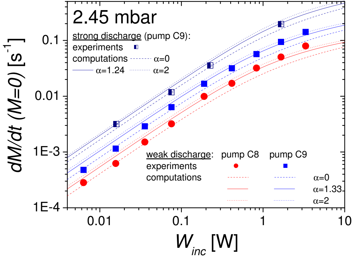
Figure 6.39: Experimental and computed time derivative of polarisation at M = 0 and p_3 = 2.45 mbar as function of incident pump laser power. Circles: pump on C 8 transition, squares: pump on C 9 transition. Filled symbols: weak discharge, half-filled symbols: strong discharge. (Experimental errors are smaller than size of symbols.) Fixed \gamma_r^P -value used in computations: (1.25 \times 10^{-7} \text{ s})^{-1} . Different assumptions of \alpha : dashed lines: \alpha = 0 , solid lines: \alpha = 1.24 (strong discharge) or \alpha = 1.33 (weak discharge), dotted lines: \alpha = 2 . Parameters of weak and strong discharges: see caption of figure 6.35.
