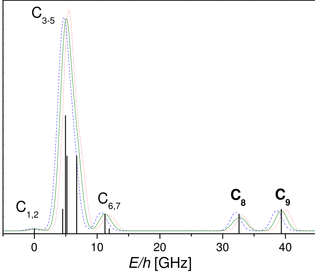
Figure 4.2: Frequencies and intensities of optical transitions in ^3\text{He} at B = 0 (vertical lines, from [Cou02]). Frequencies are referenced to the C_1 transition. The given intensities correspond to the partial sums of the transition matrix elements T_{ij} for each line.
