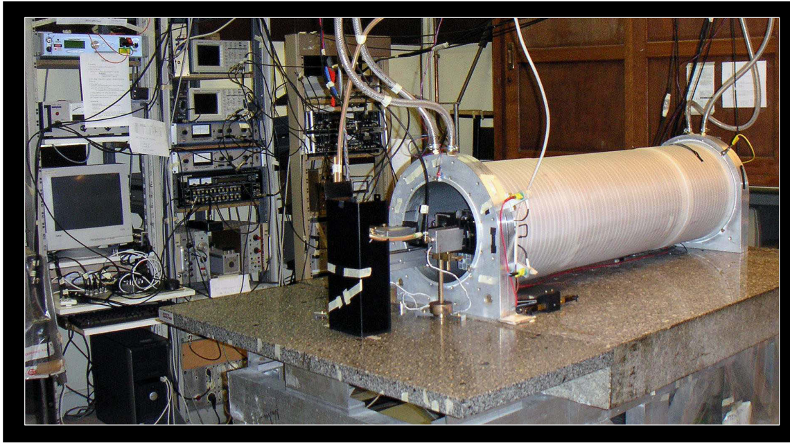
Figure 3.1: Overview of the experimental setup: In the front: End-compensated solenoid containing the optical setup (see figure 3.4). In the background: Left: Broad-band 5 W fibre laser and data acquisition system. Centre: Monitoring equipment and lock-in amplifier for transmitted pump signal. Right: Control unit and current feed of probe laser, lock-in amplifiers for transmitted probe signals, discharge generator and amplifier.
