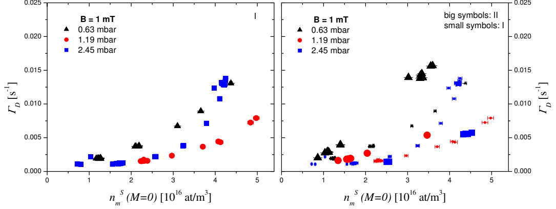
Figure 6.5: Decay rates in a plasma as function of metastable density from the present work, at M = 0 , B = 1 mT and p_3 = 0.63 mbar (triangles), 1.19 mbar (circles) and 2.45 mbar (squares). Left: Results from data-acquisition phase I only. Right: Results from data-acquisition phases II (big symbols) and I (small symbols). Experimental error bars are only visible on small symbols, in all other cases, their size is of the same order as the symbol size.
