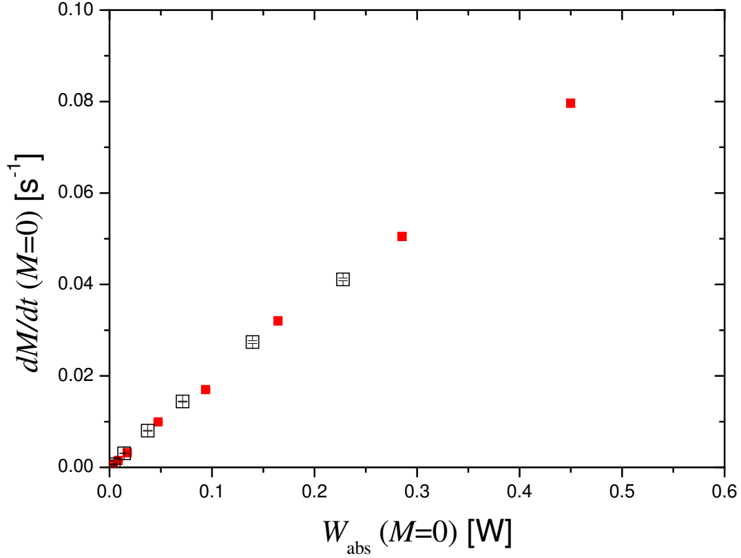
Figure 6.58: Time derivative of polarisation at M = 0 for \text{C}_8 -pumping at 2.45 mbar as a function of absorbed pump laser power at M = 0 , weak discharge (parameters: see caption of figure 6.60). Filled (red) squares: B = 1 \text{ mT} , open (black) squares: B = 30 \text{ mT} . Errors in y-direction ( \dot{M}(0) ) are plotted (barely visible in filled symbols); relative errors in x-direction on W_{\text{abs}}(0) are observed to range between approximately 1 and 5 % at the lowest investigated pressure in this work of 0.65 mbar and are smaller at higher pressure due to better SNR and a more precisely determined pump transmission coefficient at M = 0 .
