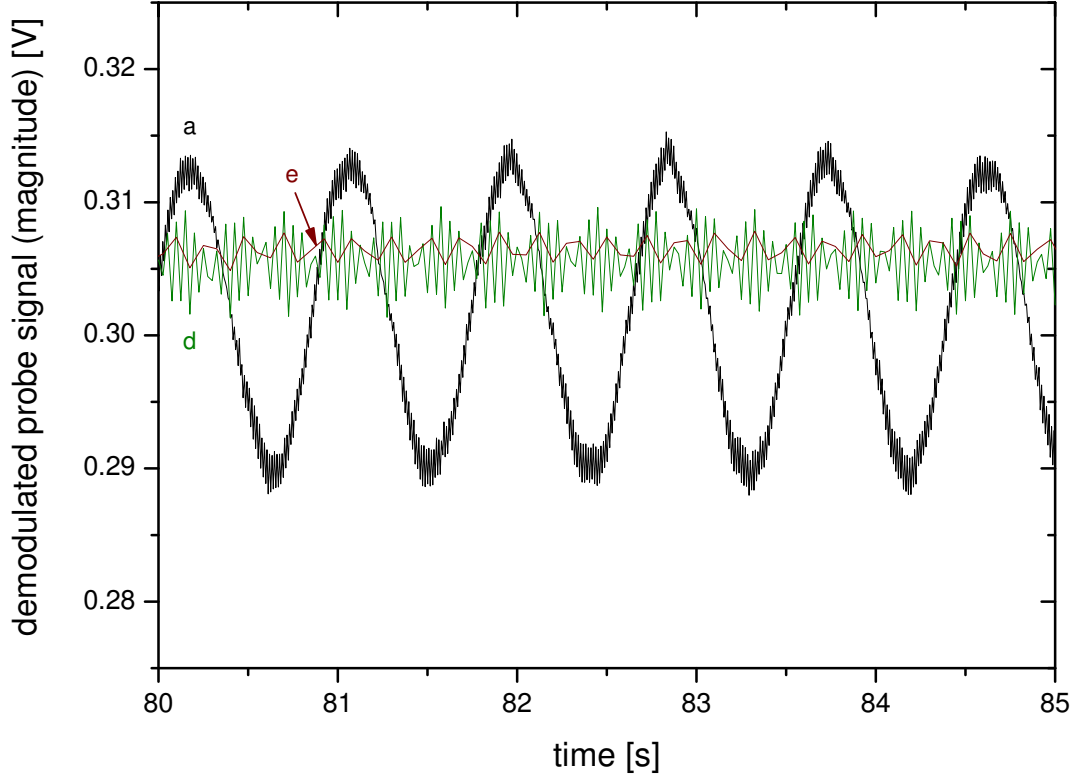
Figure E.5: Comparison of demodulated \sigma^- probe signals (simplified approach) processed with different time constants: Line a : \tau = 30 ms, line d : \tau = 100 ms and line e : \tau = 300 ms. Identical raw data in all cases: 'standard' example with W_{\text{inc}} = 0.42 W, further experimental parameters: see figure E.1.
