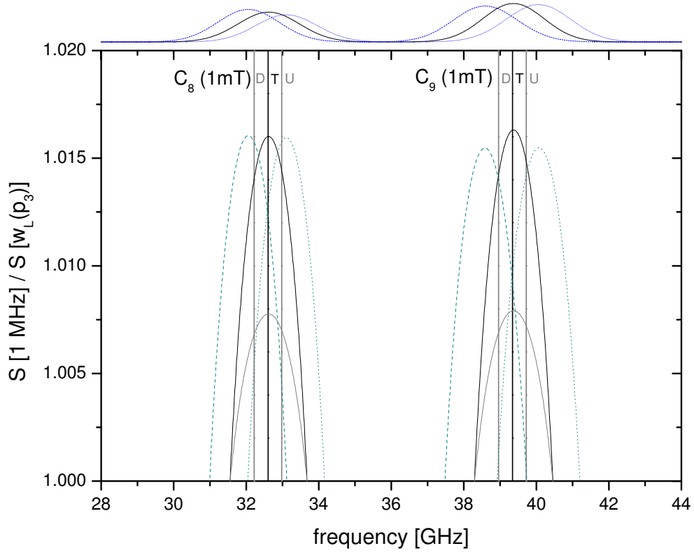
Figure 4.20: Ratio of transition intensities of Gaussian line shape divided by S(\omega/2\pi) of pressure broadened Voigt profile as function of probe frequency. Solid lines: B = 1 mT, p_3 = 1.33 mbar ( w_L = 18 MHz) and 2.67 mbar ( w_L = 36 MHz). Dashed lines: B = 30 mT, \sigma^- , p_3 = 2.67 mbar, dotted lines: B = 30 mT, \sigma^+ , p_3 = 2.67 mbar. T ('tuned'): The two dark vertical lines designate the resonance frequencies C_8 (left) and C_9 (right); D ('down') and U ('up'): the two lighter lines below and above each resonance frequency mark a possible realistic detuning range of \pm 0.38 GHz. In addition, Gaussian profiles at B = 1 mT, B = 30 mT, \sigma^- and B = 30 mT, \sigma^+ from figure 4.19 are plotted above the main graph.
