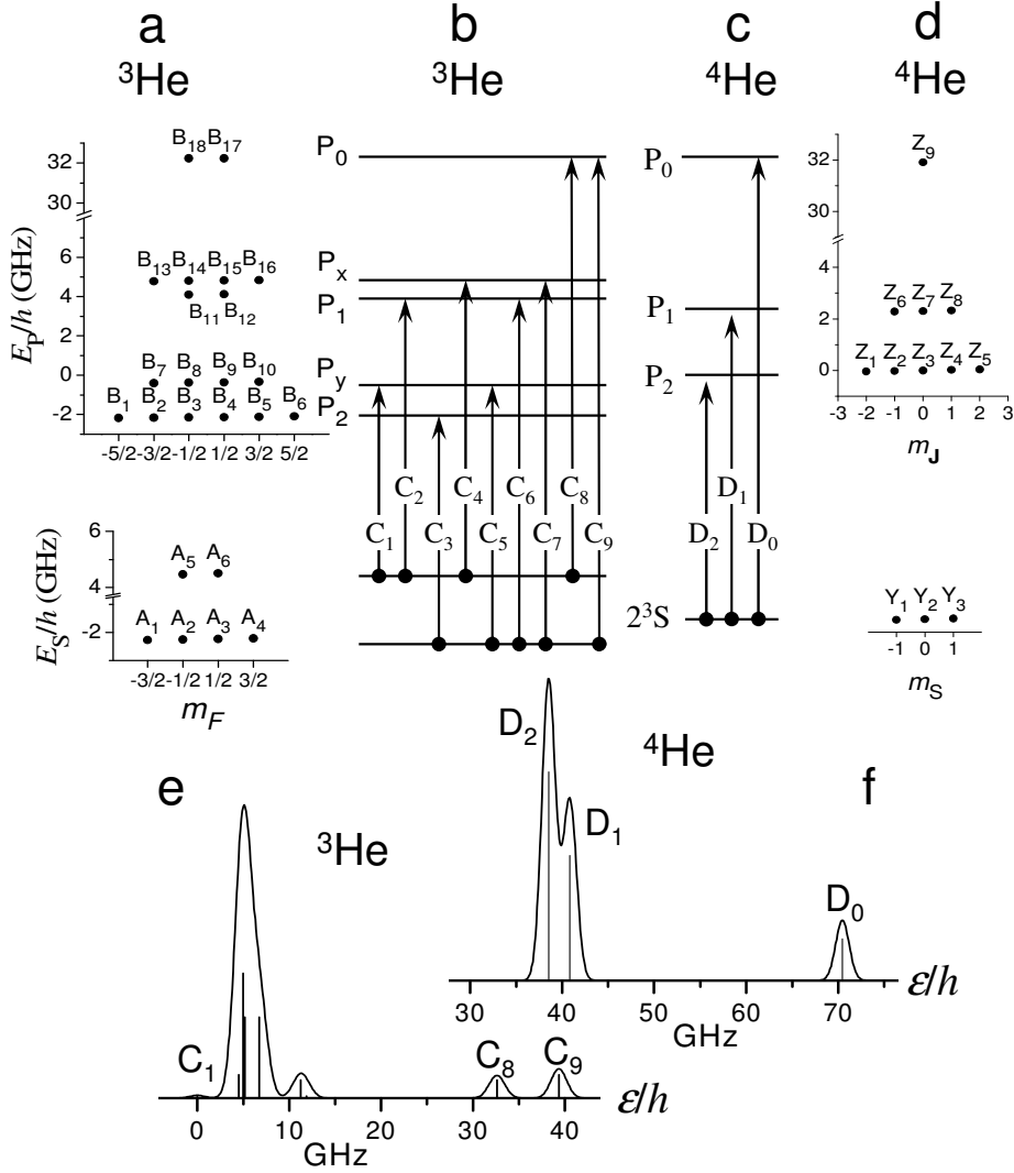
Figure 2.2: Structure of the 2^3\text{S} and 2^3\text{P} states of ^3\text{He} and ^4\text{He} and components of the 1083 nm optical transition at low magnetic field (for negligible Zeeman effect, e.g., B \leq 10 mT). a: Plot of the energies of the six 2^3\text{S} sublevels and of the eighteen 2^3\text{P} sublevels of ^3\text{He} as a function of their total angular momentum projection m_F . b: Diagram and e: Spectrum of the 9 allowed components of the 1083 nm transition of ^3\text{He} . c: Diagram and f: Spectrum for ^4\text{He} (3 line components).
