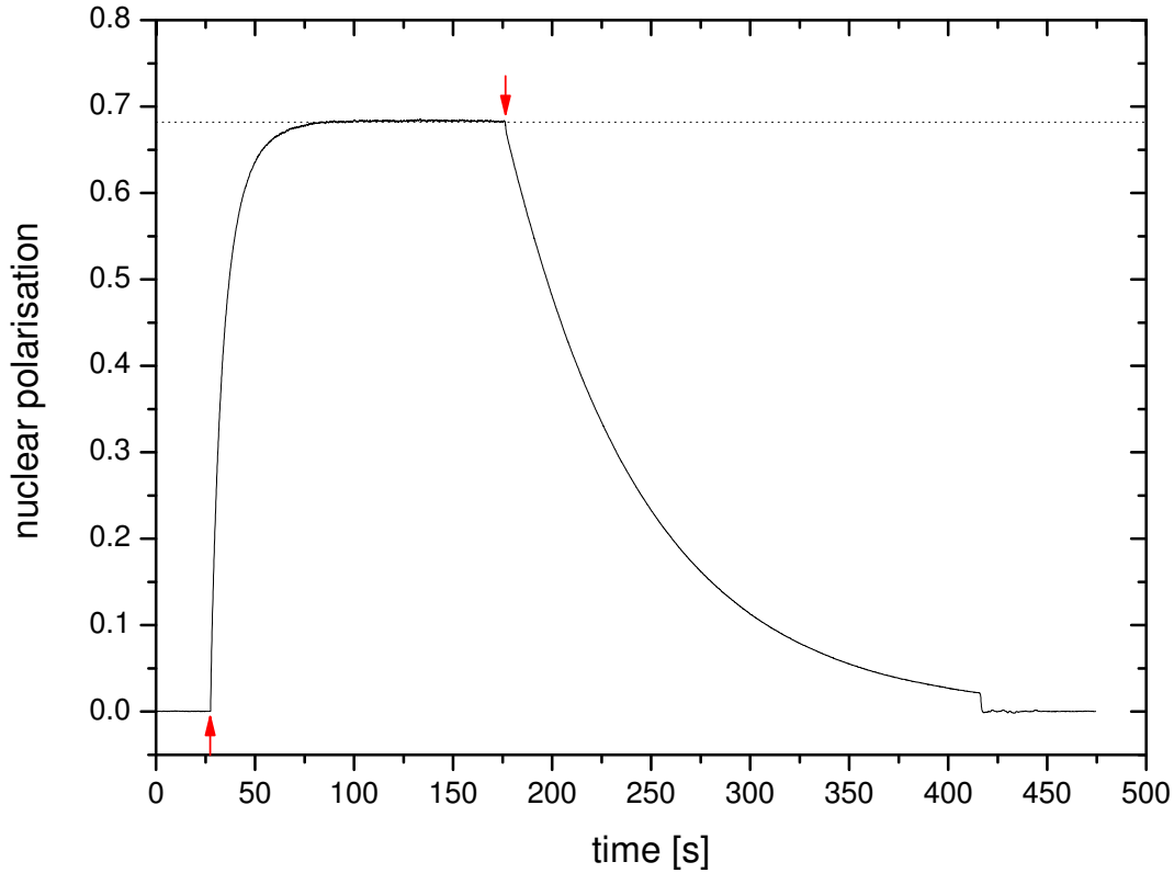
Figure 5.10: Polarisation build-up and decay at p_3 = 0.63 mbar, pump: \text{C}_8 , W_{\text{inc}} = 0.42 W, probe: \text{C}_8 , B = 1 mT, \Gamma_D = (69 \text{ s})^{-1} , n_m^S(0) = 3.34 \times 10^{16} atoms/ \text{m}^3 , data acquisition frequency: 1 kHz, signals averaged by the time constant of the numerical demodulation: \tau_{\text{LIA}} = 300 ms; no periods with discharge switched off during this acquisition; arrow at t = 27 s: pump switched on, arrow at t = 176 s: pump switched off, dotted line: M_{\text{eq}} = 0.682 , nuclear polarisation during build-up = actual polarisation (i.e., corrections to account for perturbations of 2^3\text{S} - and 2^3\text{P} -populations due to the pump laser are already applied, cf. subsection 5.3). At t = 417 s (up to t = 447 s), a magnet has been positioned close to the cell in order to record the final M = 0 level.
