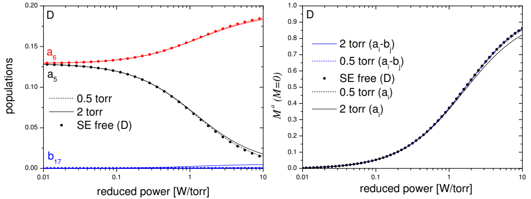
Figure G.3: Populations (of strongly pumped velocity class only) and apparent polarisation at M = 0 (probe C_8 ) as function of reduced incident power (pump C_8 ) for full collisional redistribution in 2^3\text{P} (Dehmelt-regime): The same cases of different pressure-values and assumptions to infer M^a including the SE free case as in figure G.2 are represented.
