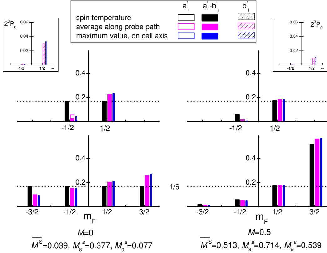
Figure 4.18: Computed OP light-induced changes in ^{23}\text{S} and ^{23}\text{P}_0 populations of the strongly pumped velocity class at p_3 = 1.33 mbar and B = 50 \mu\text{T} , for two values of M : On the left: M = 0 , on the right: M = 0.5 . Lower plots: ^{23}\text{S} populations a_1^* to a_4^* ( F = 3/2 ), upper plots: ^{23}\text{S} populations a_5^* and a_6^* ( F = 1/2 ). Insets: ^{23}\text{P}_0 populations b_{18}^* and b_{17}^* . Black (left) bars: ST populations in the absence of OP. Blue (right) bars: Example of modified populations on the axis of the Gaussian pump beam ( C_8 \sigma^+ pumping, W_{\text{inc}} = 5 W, 1.33 cm FWHM diameter, 1.7 GHz FWHM spectral width; uniform n_m = 3.2 \times 10^{16} at/m 3 , L_{\text{path}} = 2 \times 30 cm). Magenta (central) bars: Modified populations along the inclined probe path at otherwise identical conditions. For the two examples of modified populations in ^{23}\text{S} (on axis and along the inclined probe path), a_i^* (open bars) and differences a_i^* - b_j^* (filled bars) are represented. Differences are most visible for A_5 , the sublevel addressed by the \sigma^+ pump.
