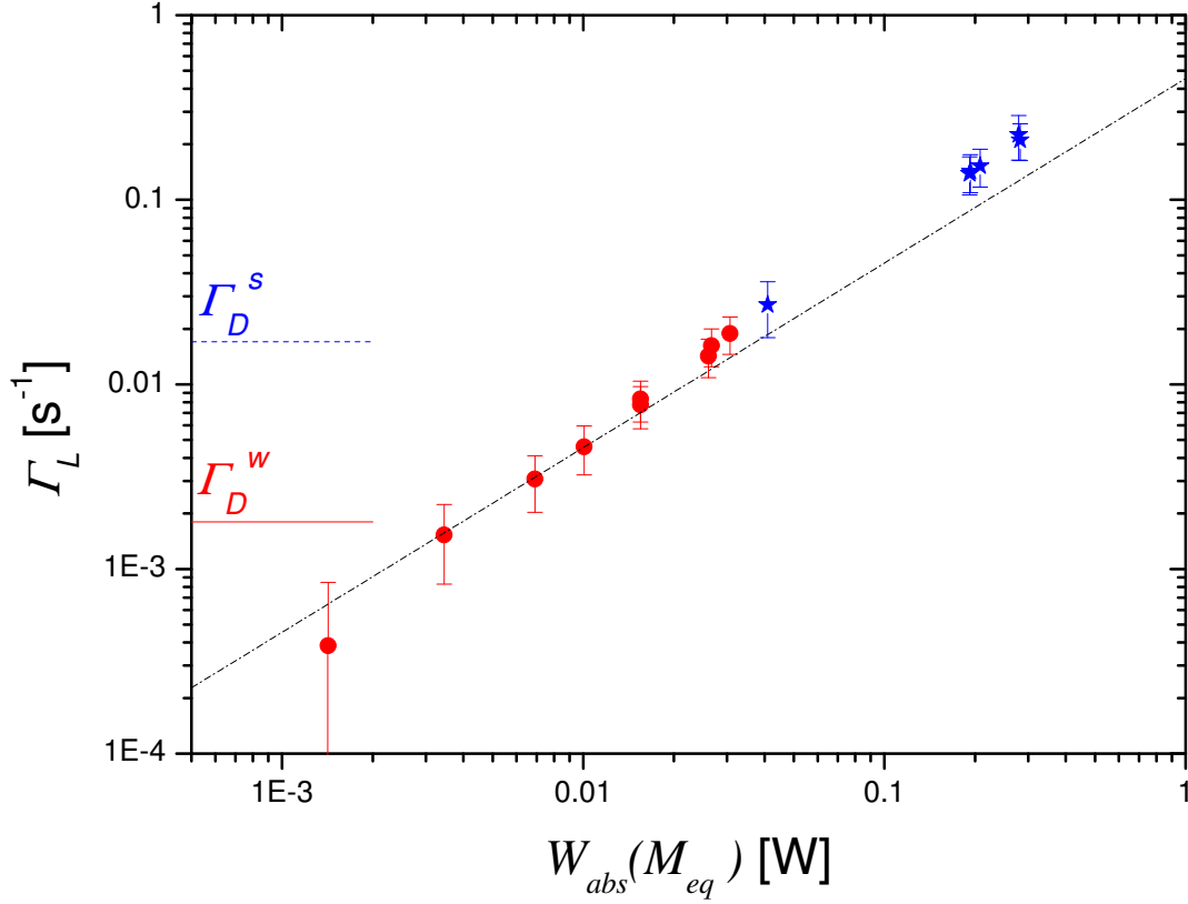
Figure 6.52: Difference between total relaxation rate \Gamma_R and decay rate \Gamma_D ( \Gamma_R - \Gamma_D = \Gamma_L ) at steady state polarisation M_{eq} at p_3 = 1.19 mbar, B = 1 mT and OP on C_8 as function of absorbed laser power. (Red) circles: weak discharge (parameters see caption of figure 6.50), (blue) stars: strong discharge, n_m^S(M = 0) = 5.7 \times 10^{16} atoms/m 3 , \Gamma_D^s = 0.017 s -1 . Dash-dotted line: guide for the eye ( y = x/2.2 ) from figure 6.50. Errors in x-direction on W_{abs}(M_{eq}) are smaller than at 0.63 mbar due to higher SNR of the pump transmission coefficient at 1.19 mbar.
