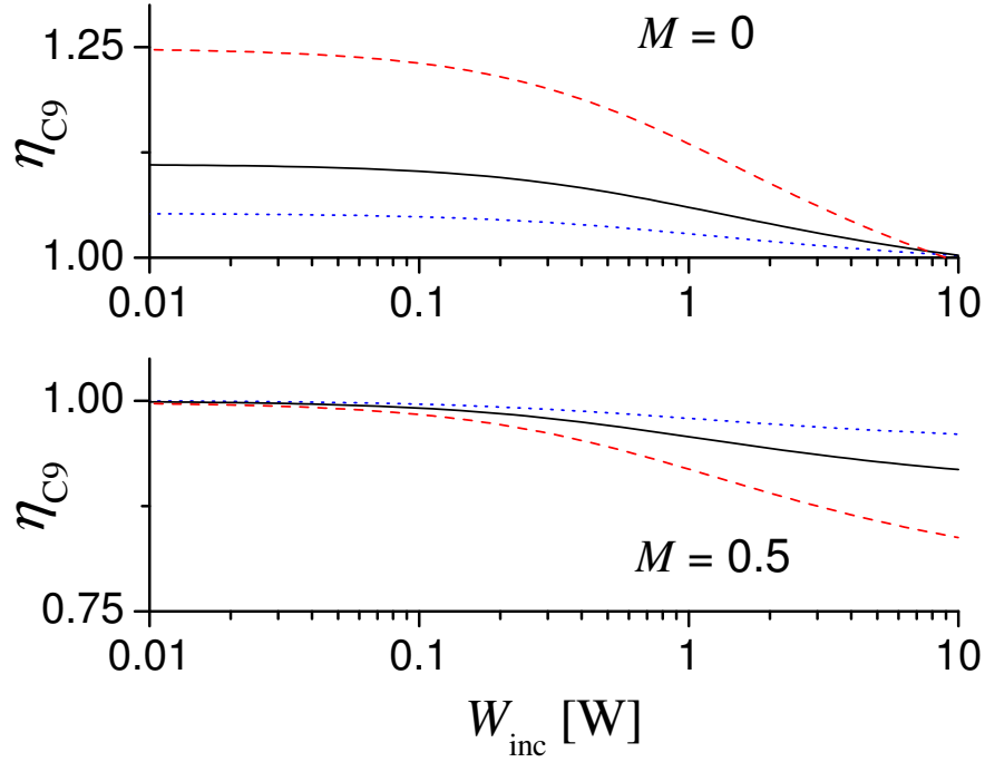
Figure 2.17: Computed power dependence of the photon efficiency of the C_9 line at M=0 (upper graph) and M=0.5 (lower graph) for the same three collisional regimes as in figure 2.14. \eta_{C9} is here the spatial average of the photon efficiency in the cell, computed for the following pump beam parameters: C_8 \sigma^+ pumping, 1.33 cm FWHM diameter, 1.7 GHz FWHM spectral width; uniform n_m = 10^{-6} \times N_g = 3.2 \times 10^{16} at/m 3 ; L_{\text{path}} = 2 \times 30 cm.
