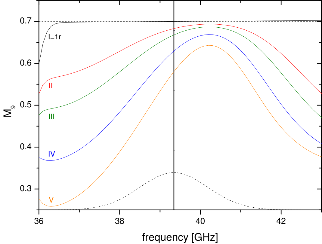
Figure 4.11: Influence of residual ^4\text{He} traces on measurement of nuclear polarisation by probe C_9 at B = 1 mT and M = 0.7 as function of probe frequency. M_9 is inferred using reduced ratios R of computed absorption signals for all different fractions x_4 of ^4\text{He} : curve I (corresponds to curve 1r of figure 4.7): pure ^3\text{He} , curve II: x_4 = 0.1 %, curve III: x_4 = 0.2 %, curve IV: x_4 = 0.5 %, curve V: x_4 = 1 %. Dashed lines: Top: Fixed M = 0.7 ; Bottom: C_9 absorption profile (not to scale) at M = 0 , B = 50 \mu\text{T} . Vertical solid line: \omega_9(B = 0) .
