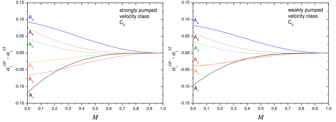
Figure 2.11: Computed OP-driven differences of populations of the 2^3\text{S} sublevels A_i with respect to ST distribution under influence of OP on the C_9 transition with W_{\text{inc}} = 1 \text{ W} , \sigma^+ light ( A_1 \rightarrow B_{18} and A_2 \rightarrow B_{17} ), pumping beam diameter: 2a = 1.6 \text{ cm} . All other parameters used for computations: see caption of figure 2.7. The displayed data correspond to the values obtained for r = 0 (i.e., along the optical axis). Left: Strongly pumped velocity class, right: weakly pumped velocity class.
