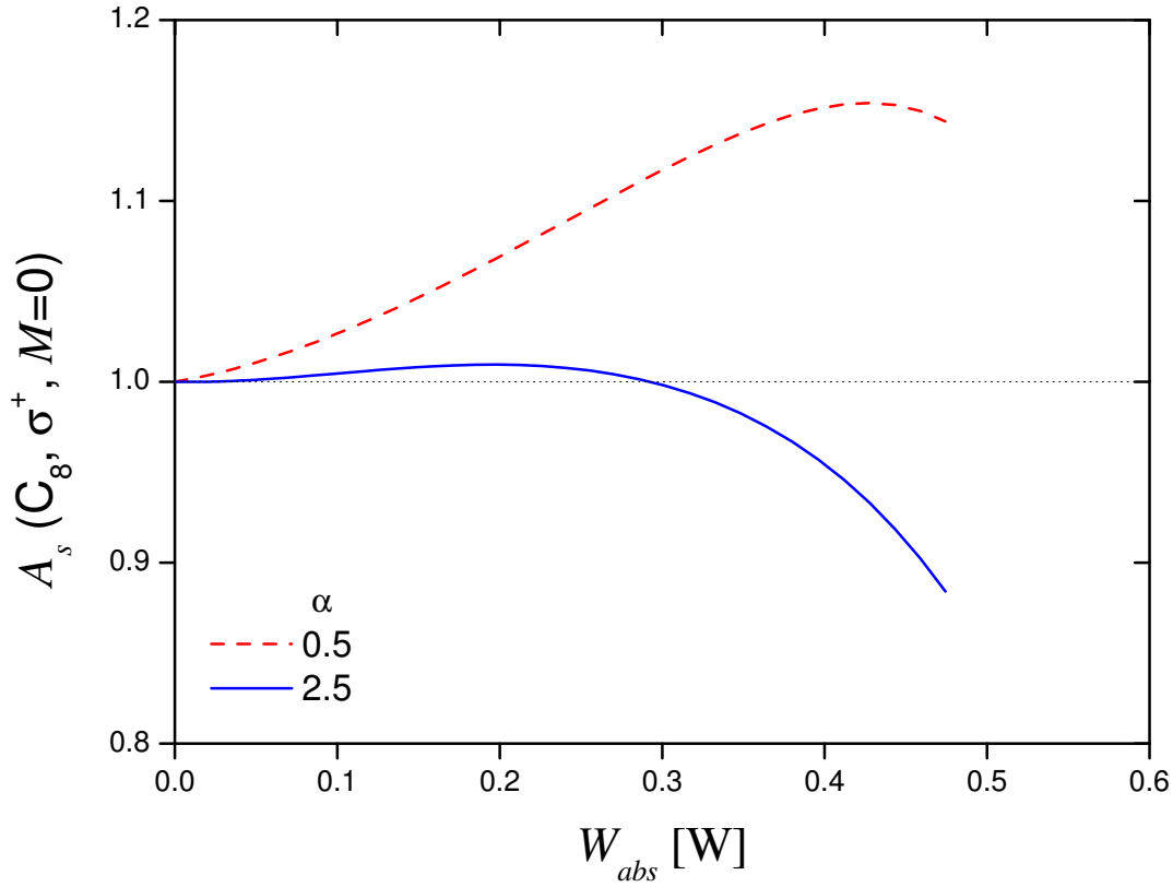
Figure 6.16: Influence of \alpha on probe absorptance A_s = 1 - T_s on C_8, \sigma^+ , at M = 0 . Relative values (at constant n_{\text{m}}^{\text{S}} ) with respect to \alpha = 0 are represented for \alpha = 0.5 (dotted line) and \alpha = 2.5 (solid line) at fixed pump beam diameter of 2a = 1.6 \text{ cm} and plotted as function of absorbed pump laser power W_{\text{abs}} . Input parameters for OP model: see caption of figure 6.15.
