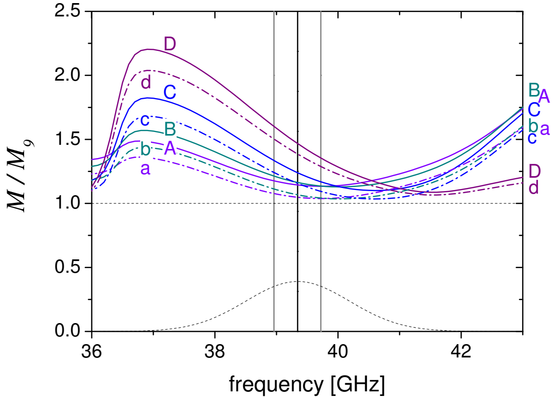
Figure 4.14: Ratios of given nuclear polarisation divided by the determined M_9 as function of probe frequency in ^3\text{He} with residual ^4\text{He} ( x_4 = 0.4 %) at B = 30 mT: M = 0.01 (a/A), M = 0.3 (b/B), M = 0.7 (c/C) and M = 0.99 (d/D).
