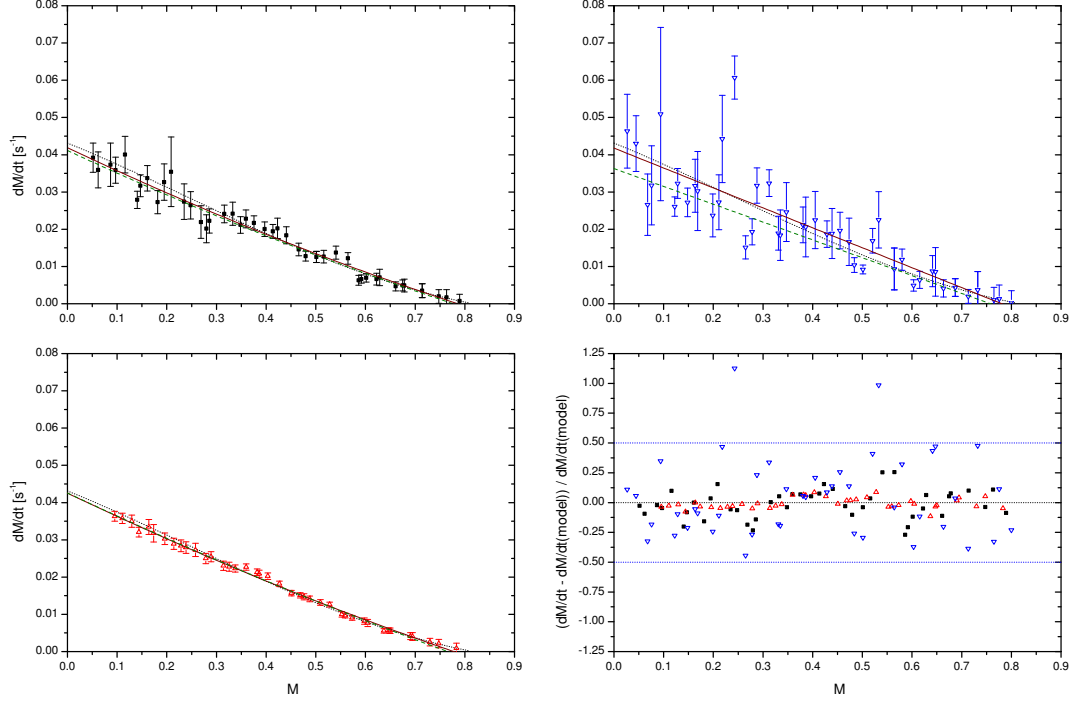
Figure F.6: \dot{M} as function of M for noisy, synthetic data without additional relaxation: Left, upper row (filled squares): Standard length of fit interval ( \frac{1}{10} of the total variation span of polarisation) in the dedicated programme. Right, upper row (open downward triangles): Short fit intervals ( \frac{1}{20} of the total variation span) in the programme. Left, lower row (open triangles): Long fit intervals ( \frac{1}{5} of the total variation span) in the programme. The dotted lines in these three graphs represent noiseless \frac{dM}{dt} -values as function of M given by the MEOP-model. The solid lines show the best polynomial fit in each case for fits without error weighting (based on the criteria mentioned above). The dashed lines represent the fits with error weighting for the same polynomial orders and the same borders of the fits as used in the case without error weighting. Right, lower row: Relative errors with respect to noiseless \dot{M} generated by the MEOP-model for all investigated lengths of fit intervals in the programme. Dotted lines in this graph: Zero- and 50 %-error-levels.
