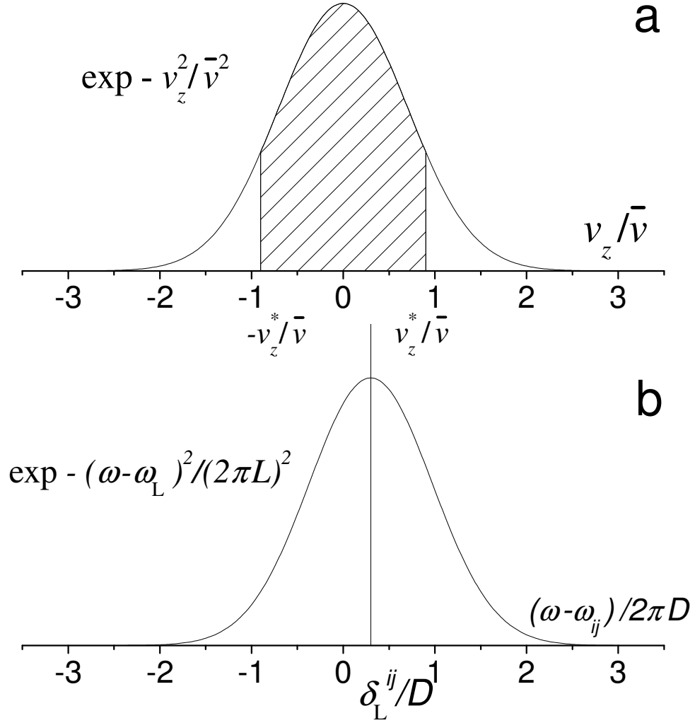
Figure 2.5: Two-class OP model. a: Maxwell velocity distribution of atoms characterised by its most probable velocity \bar{v} and Gaussian width D (see section 2.3). It is split in two broad classes using the velocity boundary v_z^* . The atoms with |v_z| < v_z^* belong to the “strongly pumped” class (hatched area); the atoms with |v_z| > v_z^* belong to the “weakly pumped” class. b: spectral profile of the pump laser (Gaussian width: L , frequency detuning: \delta_L^{ij} = (\omega_{ij} - \omega_L)/2\pi with respect to the atomic transition frequency \omega_{ij}/2\pi ).
