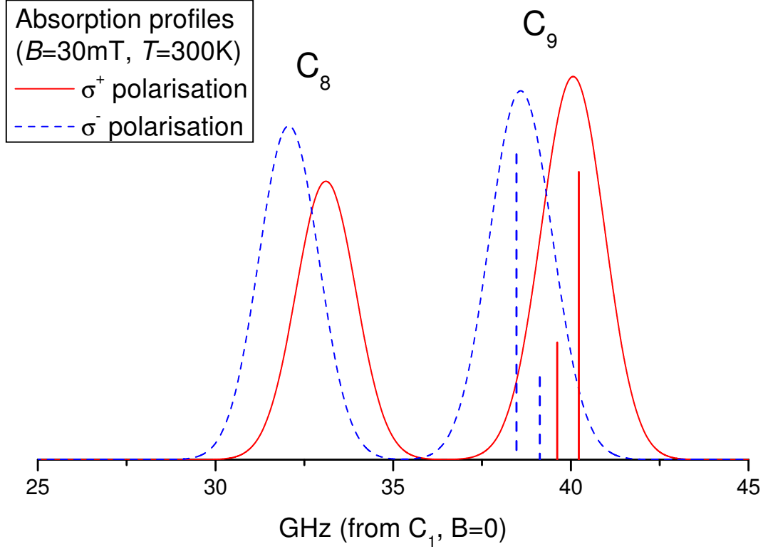
Figure 2.4: Computed ^3\text{He} C_8 and C_9 absorption spectra at null polarisation in B=30\text{ mT} for gas at room temperature with no collisional broadening. Solid (resp. dashed) lines correspond to \sigma^+ (resp. \sigma^- ) polarisation. The vertical bars (same line styles) represent the positions and amplitudes (matrix elements T_{ij} ) of the two unresolved components of the C_9 line (e.g., A_1 \rightarrow B_{17} and A_2 \rightarrow B_{18} for \sigma^+ polarisation). Transition frequencies are referenced to the frequency of the C_1 resonance at B = 0 (see text). The C_8 – C_9 splitting is equal to 6.739 GHz at B=0 (see appendix A)
