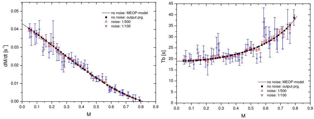
Figure F.1: Left: \dot{M} as function of polarisation. Right: T_b as function of polarisation. Both graphs represent processed data by the dedicated programme for polarisation build-up analysis. As input, synthetic data generated by the model for MEOP-kinetics (parameters see text) was used with different noise levels: Triangle: Output of programme for noise level 2 ‰ of generated random Gaussian noise (with standard deviation = 1) on M(t) . Downward triangle: Output of programme for noise level 1% of generated random Gaussian noise on M(t) . Filled squares: Output of programme for noiseless data. Continuous line: Theoretical values of \frac{dM}{dt} and T_b provided by the MEOP-model.
