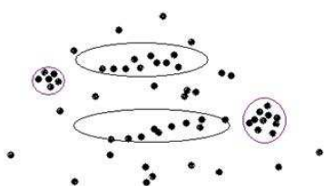
Fig 2.2 Compact and Chained clusters
