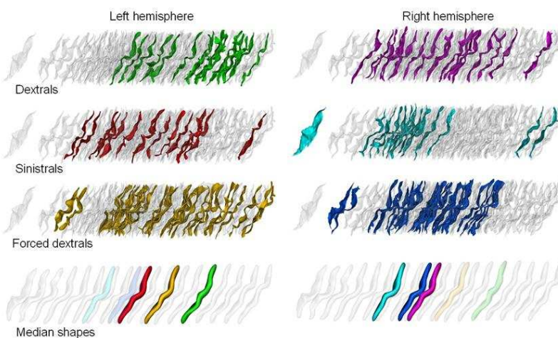
Fig 4.7 Population localization along the Isomap axis
