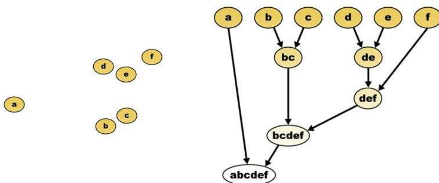
Fig 2.5 Sample data distribution and the formation of agglomerative clustering tree
