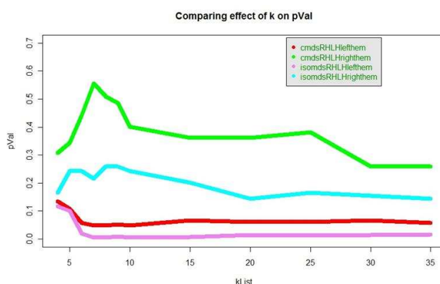
Figure 4.11 Neighbourhood size and p-value
