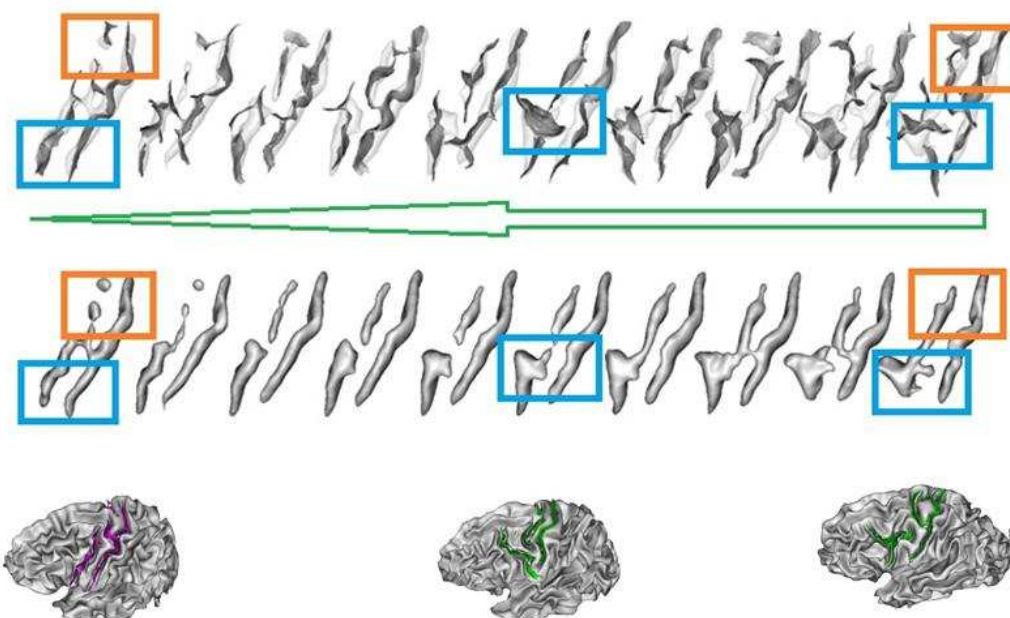
Fig 5.11 The variability model of the precentral region
