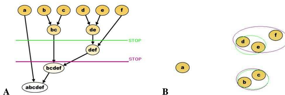
Fig 2.13. Two different stopping rules.
