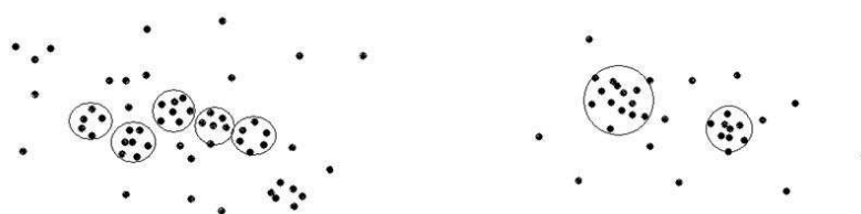
Figure 2.12 Typical clustering result of complete-linkage and average-linkage.
