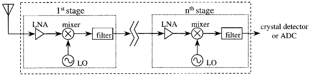
Figure 6.3.: Traditional digitization front-end, (picture from [96])
