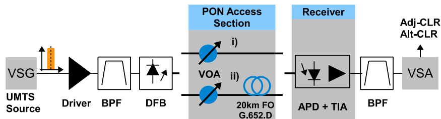
Figure 10.1.: Experimental set-up using an APD receiver
