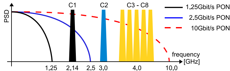
Figure 5.1.: Schematic summary of the different SCM of PON signals with radio carriers [86–89]. C1-C8 represent the different radio carriers.
