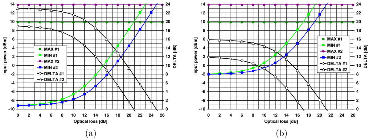
Figure 7.8.: Input powers (minimum and maximum) and power ranges assuming +5dBm (curves #1) and +7dBm (curves #2) optical launch powers for a channel width of (a) 3.84 and (b) 20MHz, when targeting a 50dB SNR.
