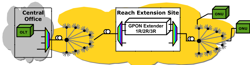
(b) Second reference architecture
