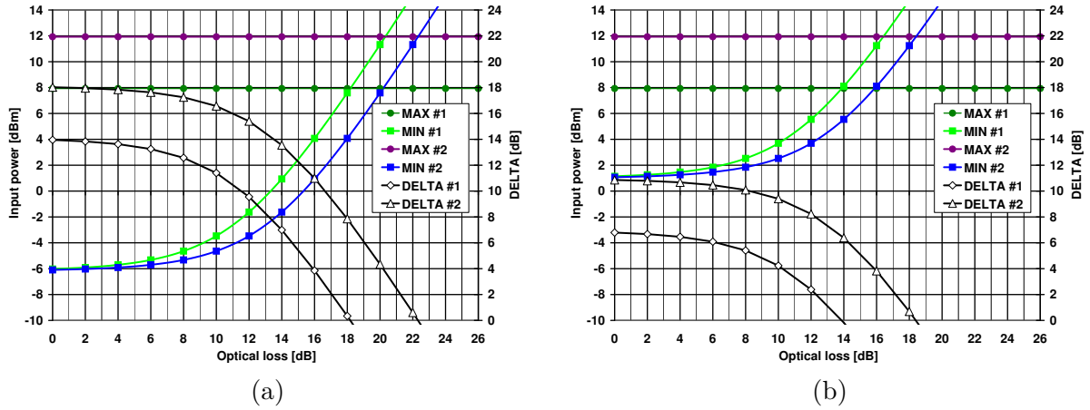
Figure 7.9.: Input powers (minimum and maximum) and power ranges assuming +5dBm (curves #1) and +7dBm (curves #2) optical launch powers for a channel width of (a) 3.84 and (b) 20MHz, when targeting an overall 50dB SNR.
