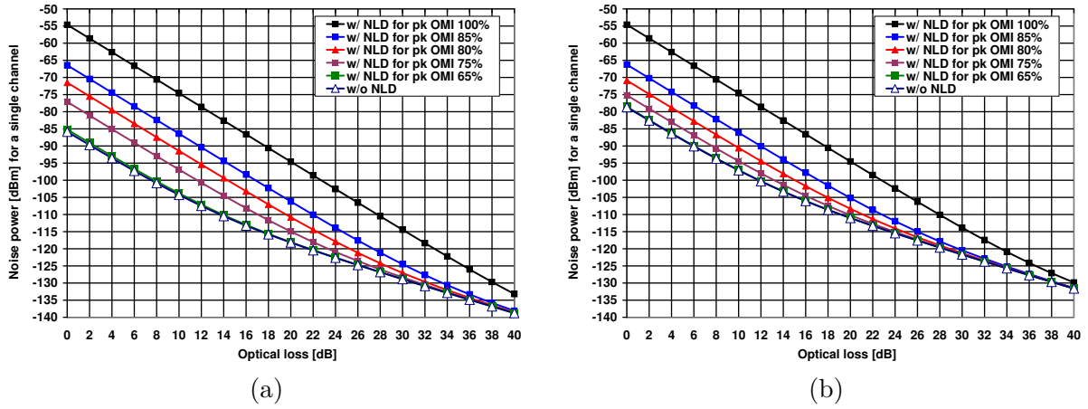
Figure 7.13.: Received noise power with and without the NLD component for several peak OMIs (10dB-crest-factor signal) for an optically amplified link, and for channel bandwidths of (a) 3.84MHz, and (b) 20MHz
