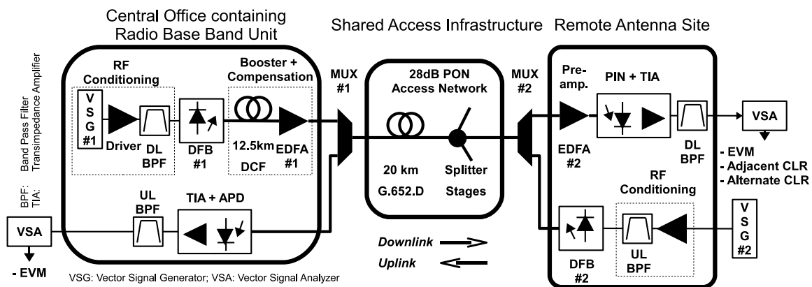
Figure 13.16.: Perspective set-up
