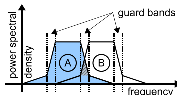
Figure 3.22.: Illustration of interferences between adjacent channels: the dashed area in the channels \text{\textcircled{A}} and \text{\textcircled{B}} are interferences caused by the respective neighbor channel.
