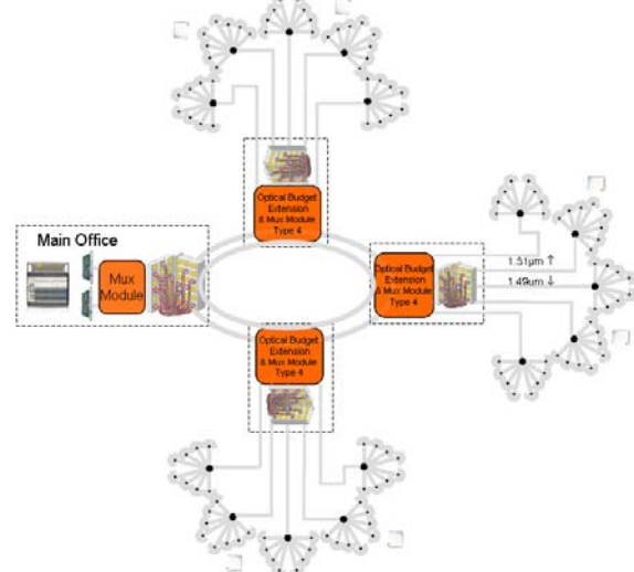
Figure 6: metropolitan and access merger approach.
