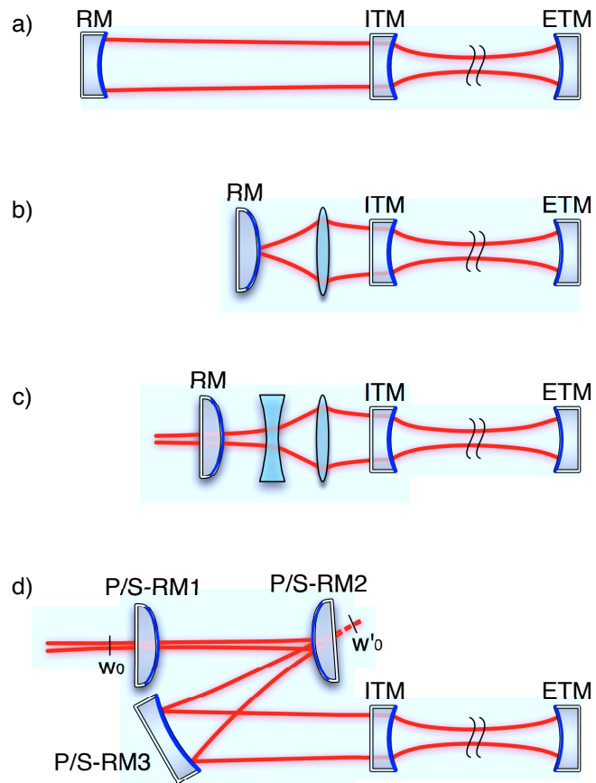
Figure 5.9: Evolution of the design concept of non-degenerate recycling cavities for AdV.
