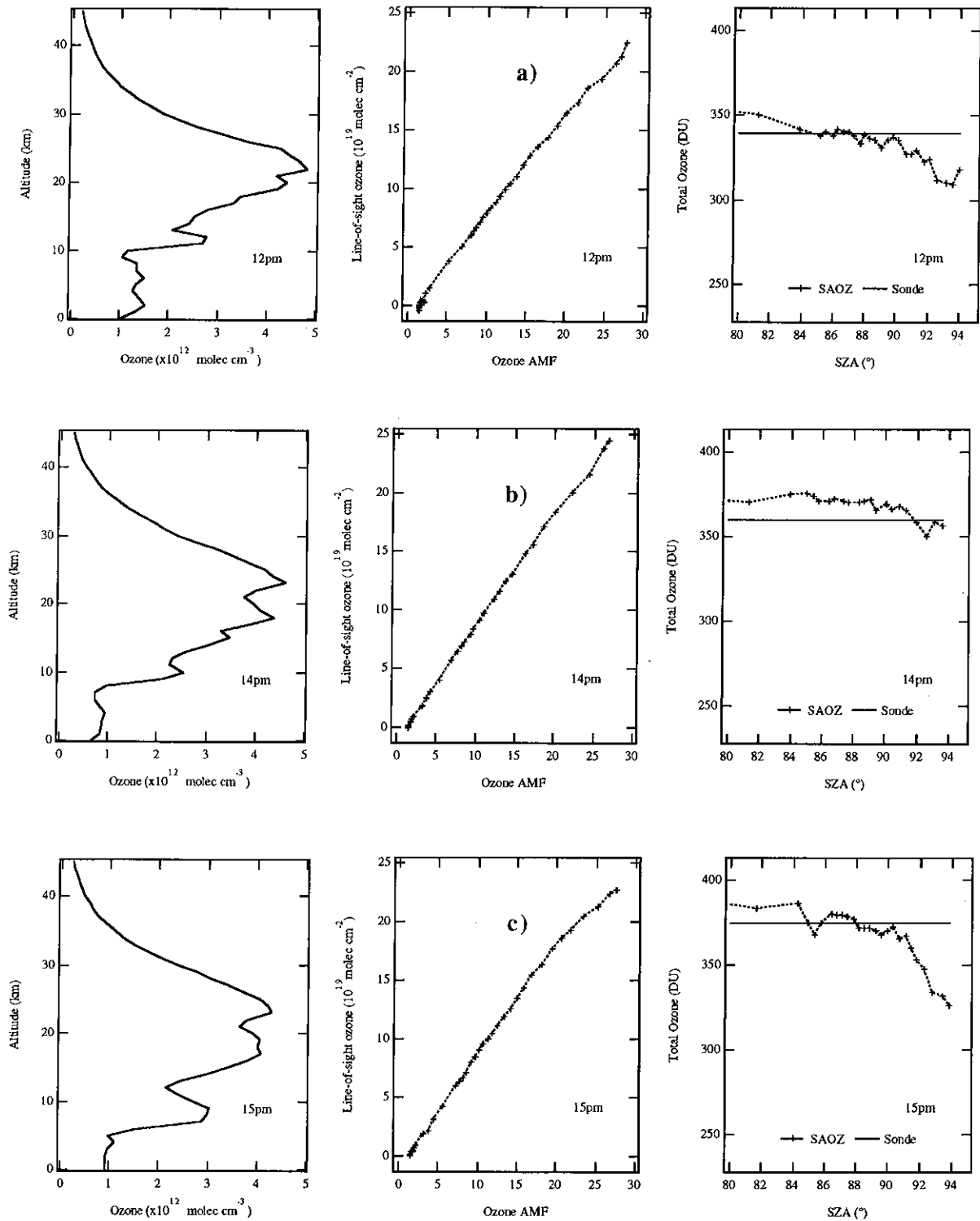
Figure 3. (a) - (k) Ozone measurements in September 1994 at Camborne, UK (50°N, 5°W). Left-hand panels: The ozone profiles from ECC ozonesondes. Values above the highest altitude of the sonde are calculated assuming a constant mixing ratio up to 90 km. Middle panels: The Langley plot for half-day periods when a sonde was flown. Measurements are from the SAOZ spectrometer which is normally stationed at Aberystwyth, UK. AMFs are calculated using measured ozone and temperature (hence density) profiles. The reference spectrum used in these SAOZ analyses is taken at noon on each day. Right-hand panels: Vertical ozone from SAOZ (crosses) using daily AMF and R_{\text{sonde}} , and from integrated sonde profiles (horizontal line). SAOZ values at \text{SZA} < 80^\circ are not shown because of their large scatter.
