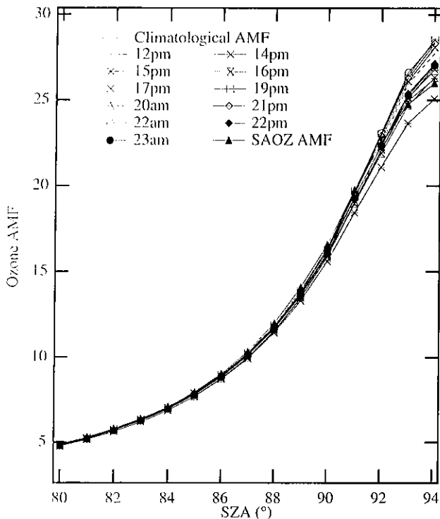
Figure 1. Ozone AMFs calculated using the ozone and density profiles measured by each ozonesonde flown in September 1994 at Camborne, U.K. ( 50^{\circ} N, 5^{\circ} W), together with the SAOZ AMF (see text).
