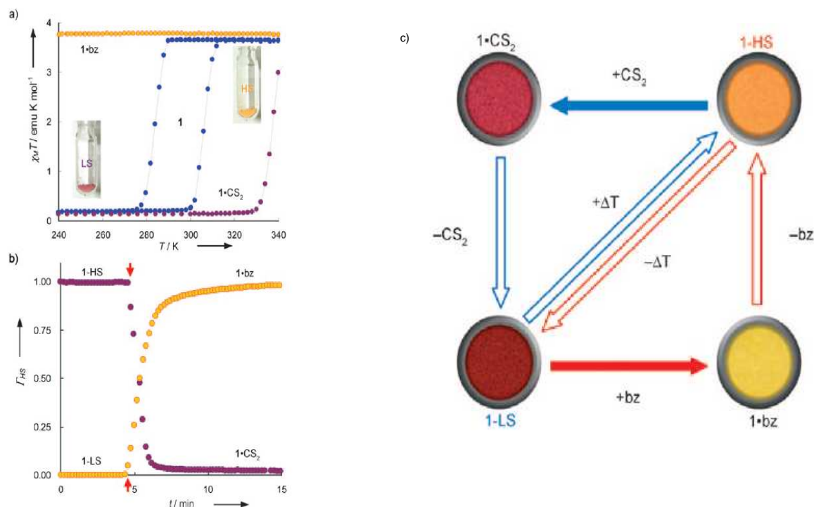
Fig.1.12: Magnetic behavior of \{\text{Fe}(\text{pz})[\text{Pt}(\text{CN})_4]\} powder and its clathrates a) Temperature dependences of \chi_M T for guest-free 1 (blue), benzene (Bz) clathrate ( 1·bz : yellow), and CS 2 clathrate ( 1·CS 2 : purple); b) Time dependence of the fraction of the HS state ( G ) under a benzene (yellow) and CS 2 (purple) atmosphere at 293 K; and c) Schematic chemical and thermal memory process. The color circles are real photos of powder samples. [Ohba 2009]
