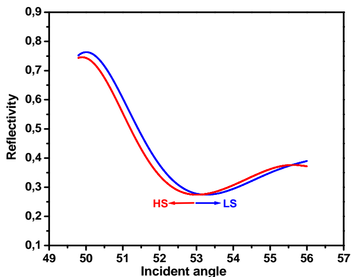
Figure.III.21: Surface plasmon resonance of the spin-coated [Fe(hptrz)_3](OTs)_2 SCO thin film on glass/Ti/Au substrate at 308 K (LS) and 343 K (HS).
