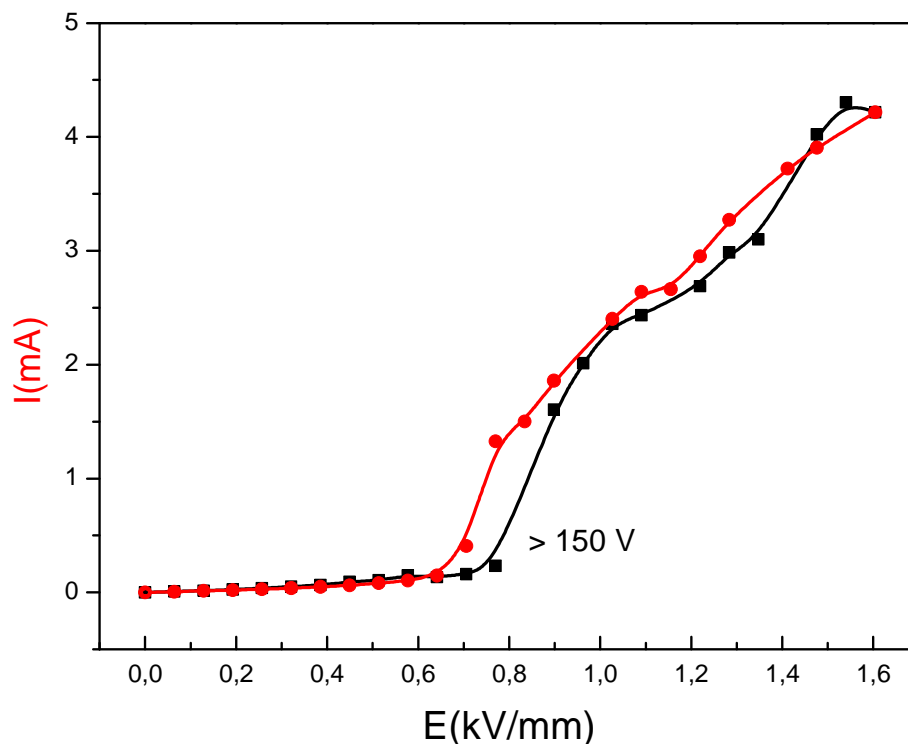
Fig.II.22: Variation of the electric current as function of the electric field applied on a stepwise manner on the compound 9 . The current increases typically from \sim 0.1 to a few mA.
