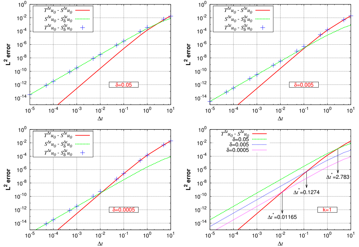
Fig. 5.1: 1D KPP equation with k = 1 . Local L^2 errors for several splitting time steps \Delta t and \delta = 0.05 (top left), 0.005 (top right), and 0.0005 (bottom left). Bottom right: critical splitting time steps \Delta t^* obtained when \|T^{\Delta t} u_0 - \mathcal{S}^{\Delta t} u_0\|_{L^2} \approx \|\mathcal{S}^{\Delta t} u_0 - \mathcal{S}_\delta^{\Delta t} u_0\|_{L^2} , in the numerical tests.
