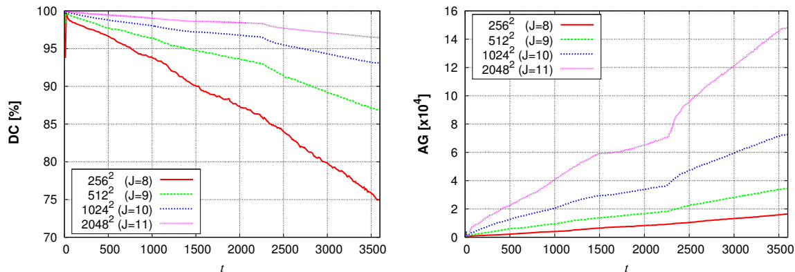
Fig. 9.17: 2D stroke model. Time evolution of data compressions DC given by (4.39) (left) and the number of points on the adapted grids AG (right) for different finest levels J .
