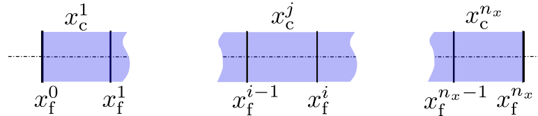
Fig. 11.4: Definition of the grid: the cell centers are located at x_c^j , whereas cell faces are located at x_f^i . The domain is bounded by faces x_f^0 (cathode) and x_f^{n_x} (tip of the anode).
