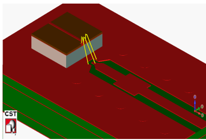
Figure 3.37: "dpatch" = 1mm
