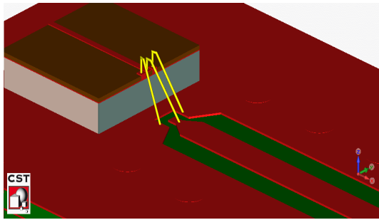
Figure 3.29: "N" = 2mm
