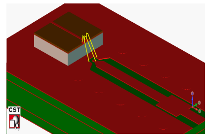
Figure 3.39: "dpatch" = 3mm
