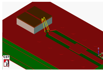
Figure 3.38: "dpatch" = 2mm
