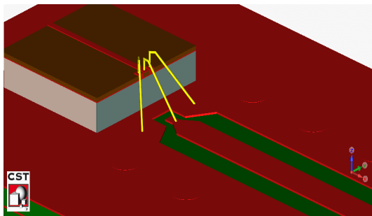
Figure 3.31: "N" = 22mm
