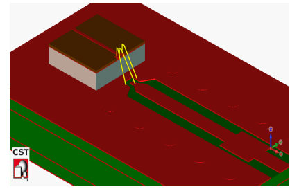
Figure 3.39: "dpatch" = 3mm
