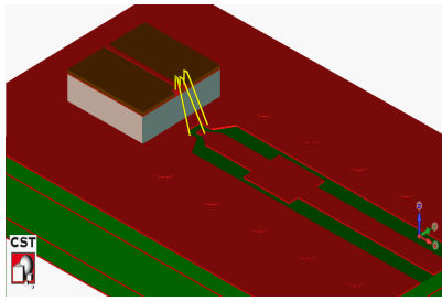
Figure 3.37: "dpatch" = 1mm
