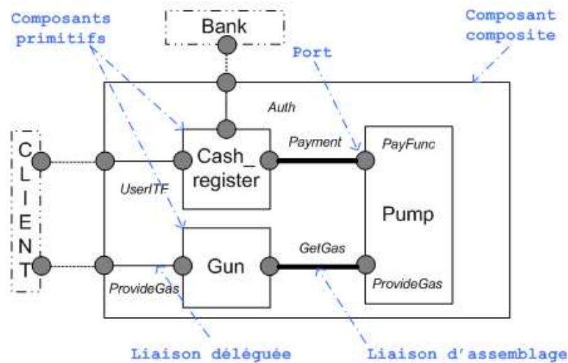
FIG. 2.6 – Architecture de station essence en SafArchie
