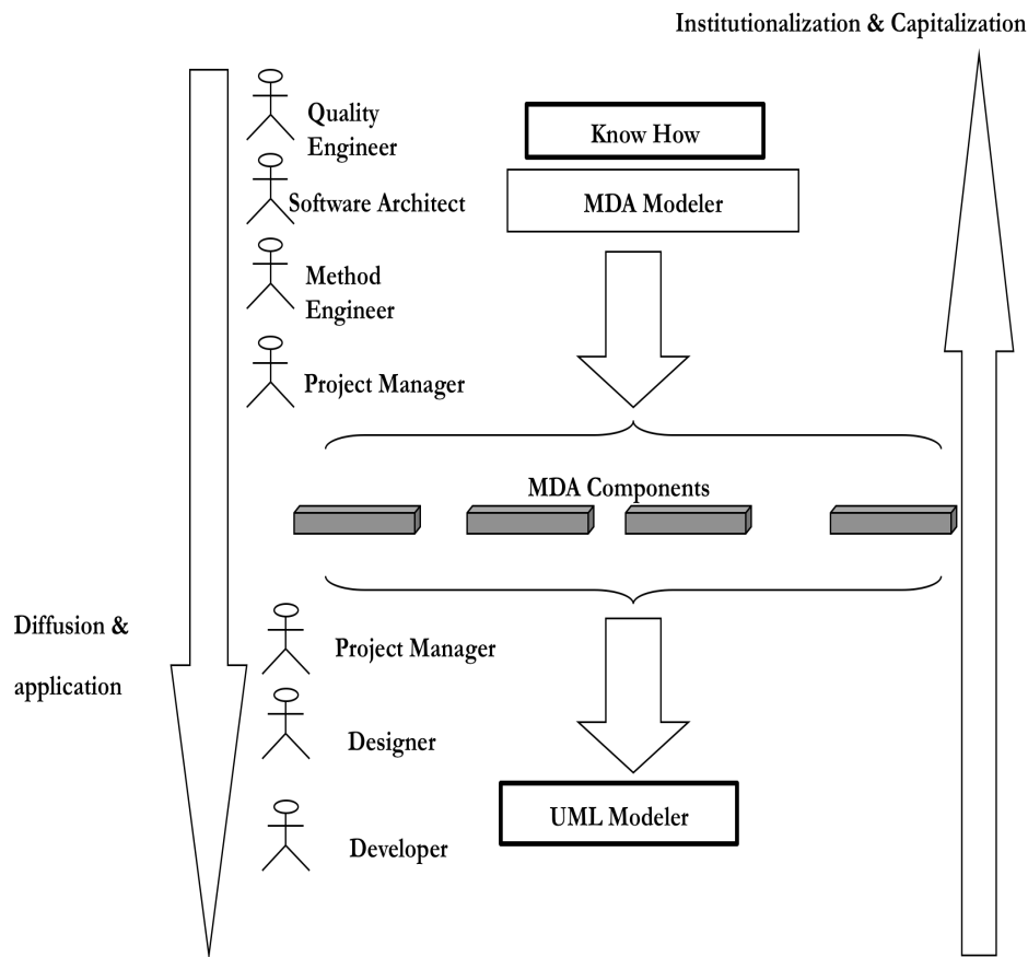
Figure II.10 Principes de MDA Modeler et UML Modeler [Softeam, 2008]
