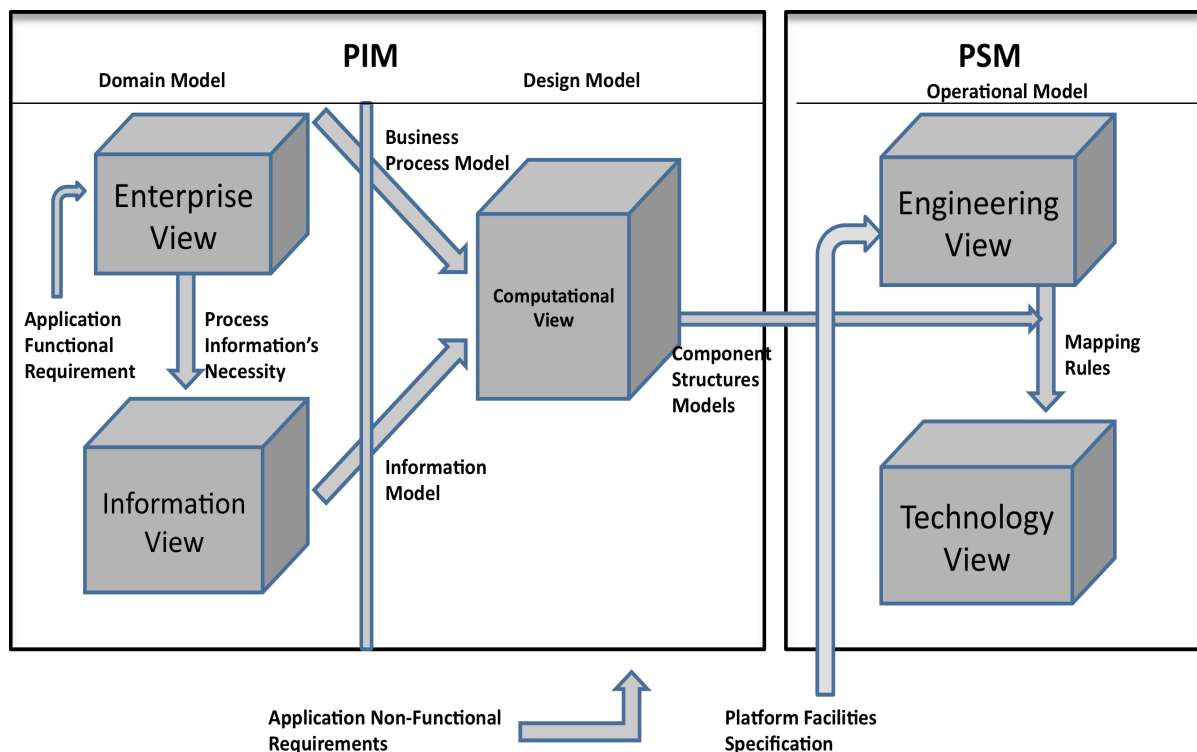
Figure II.12 Processus dédié aux services d'architectures [Maciel et al., 2006].
