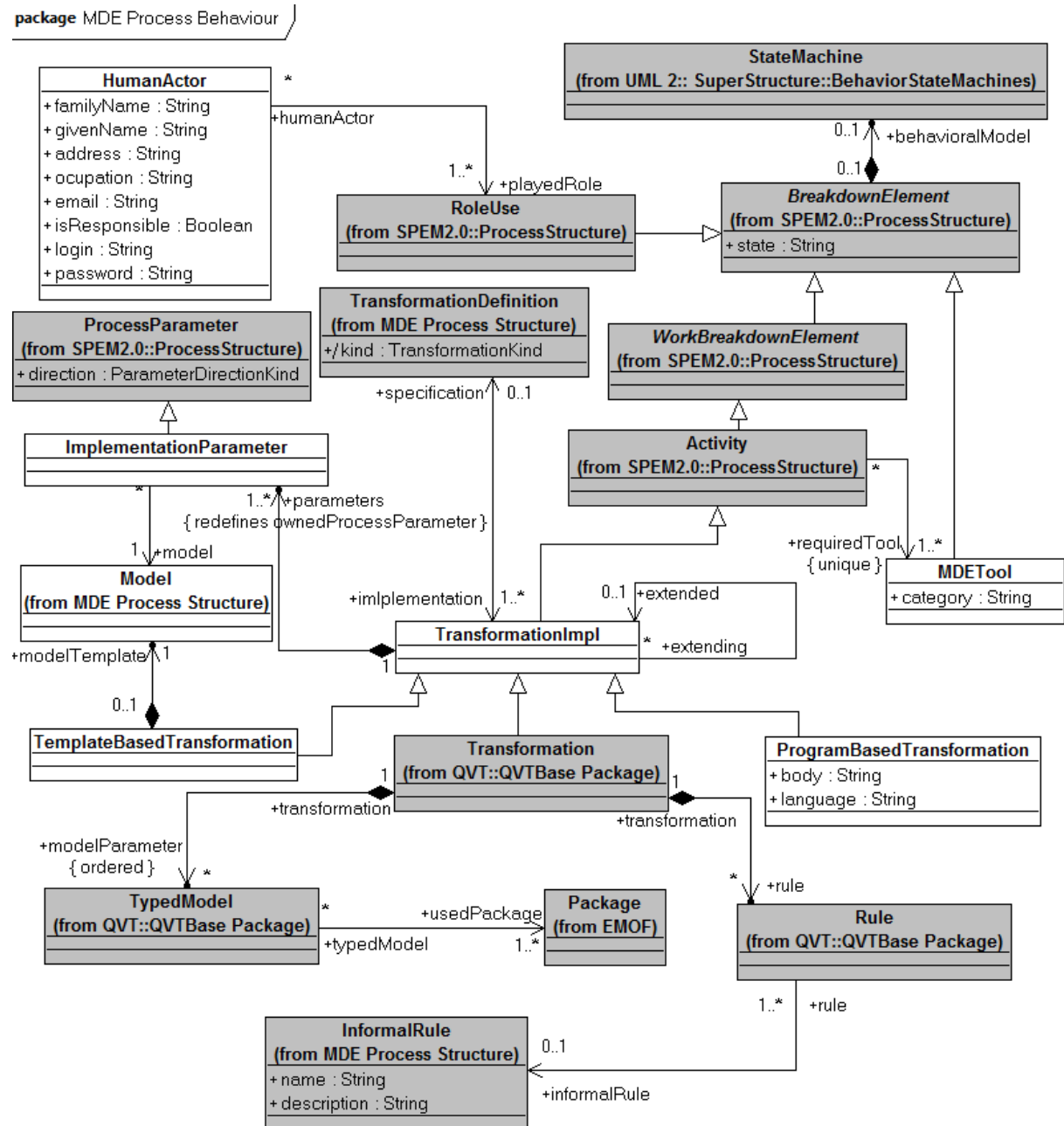
Figure III.7. Paquetage MDE Process Behavior
