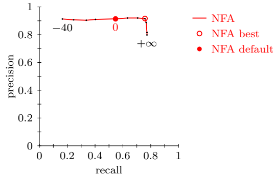
Figure 56: NFA parameter tuning on the snow sequence. The performances of the NFA algorithm with holes on the snow sequence are represented in the (recall, precision) plane in function of the threshold parameter \log_{10} \varepsilon . While the precision remains merely constant, a good recall is obtained by the default value (0) of \log_{10} \varepsilon , but the results can be improved by choosing a slightly greater value ( \log_{10} \varepsilon = +5 , that corresponds to the “NFA best” point).
