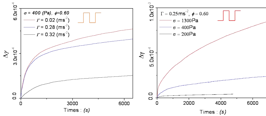
FIGURE 4.6: Creep deformation with square tension input and packing fraction \phi = 0.60 , for different vibration levels at applied shear stress \sigma = 400Pa (left) and for different applied shear stresses at r.m.s vibration \Gamma = 0.25ms^{-2} (right).
