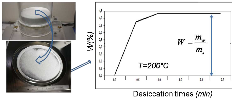
FIGURE 2.24: Granular sample and dessicator interior (left) and the water content W\% as a function of desiccation times with 200^\circ\text{C} , the plateau corresponded to the mass of dry grains (right).
