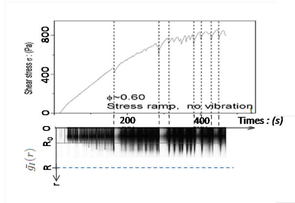
FIGURE 3.32: Response to a stress ramp on the sample surface. Shear stress as a function of times for a packing fraction \phi = 0.60 and \dot{\beta} = 0.00052rd/s with the juxtaposing of \bar{g}_I(r)
