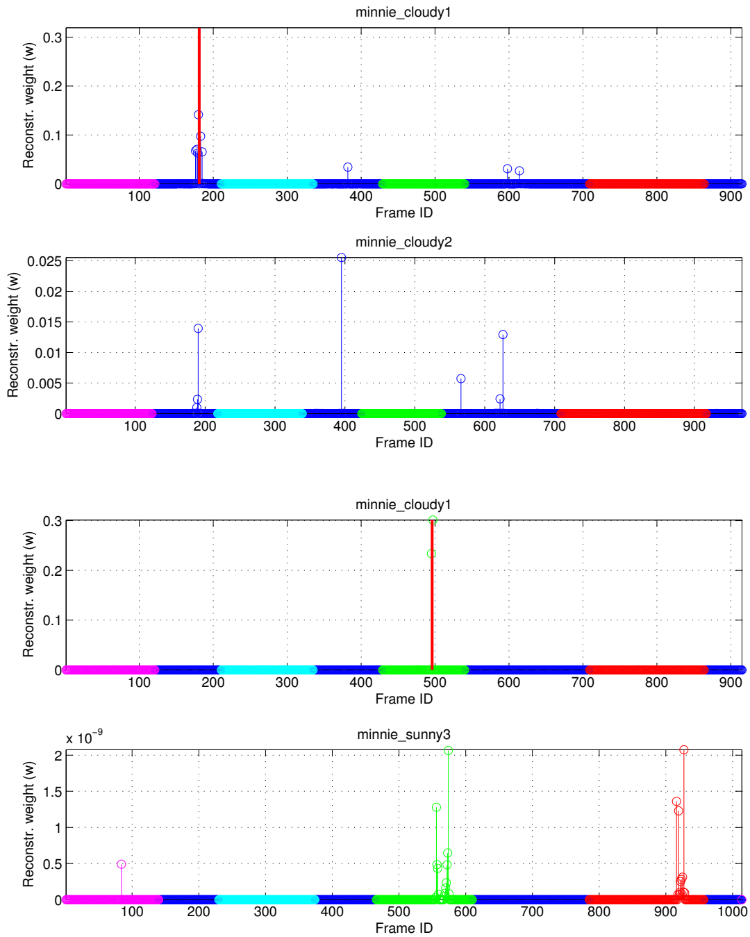
Figure 4.16: Label Propagation - Graph links found using the LNP algorithm (top) EASY: from cloudy1 to cloudy2 (bottom) HARD: from cloudy1 to sunny3; Best viewed in color.
