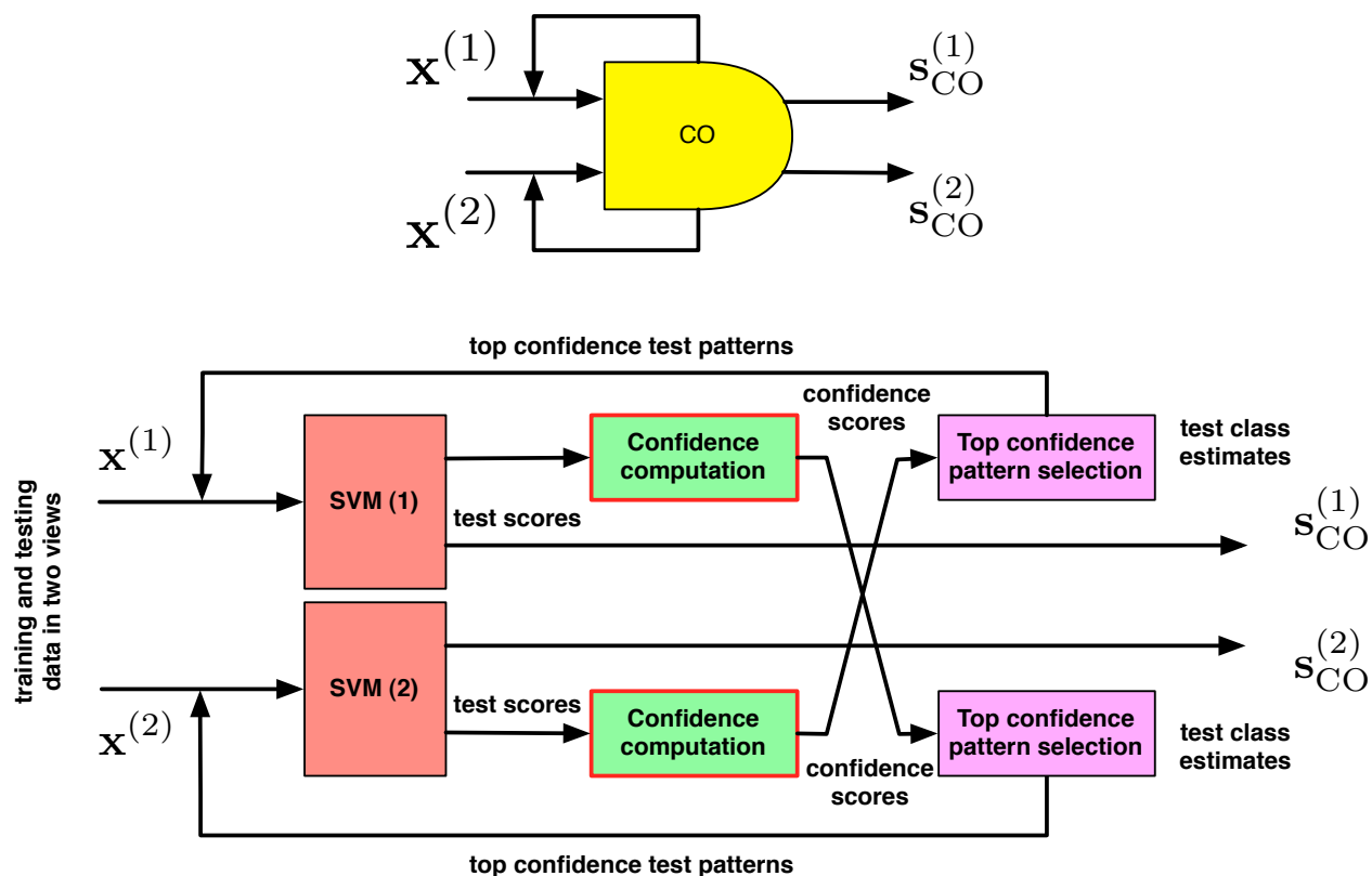
Figure 4.4: Co-Training module
