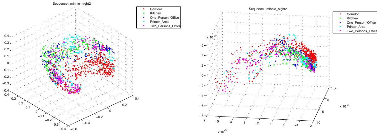
Figure 2.3: KPCA (left), LapEig (right) : Sequence “minnie_night2” with class information
