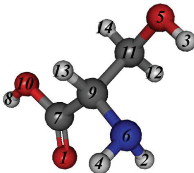
Figure 3.18: Lowest-energy structure of the solvated serine, optimized at the B3LYP/6-311++G** level
