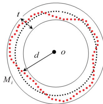
Figure 3-29: Cylindricity tolerance zone
