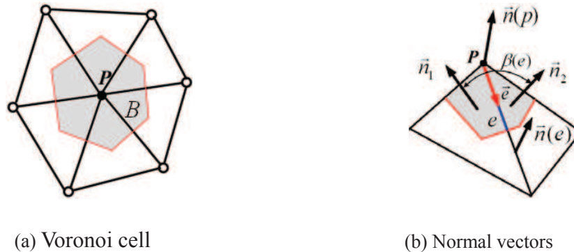
Figure 3-7: Discrete curvature estimation parameters
