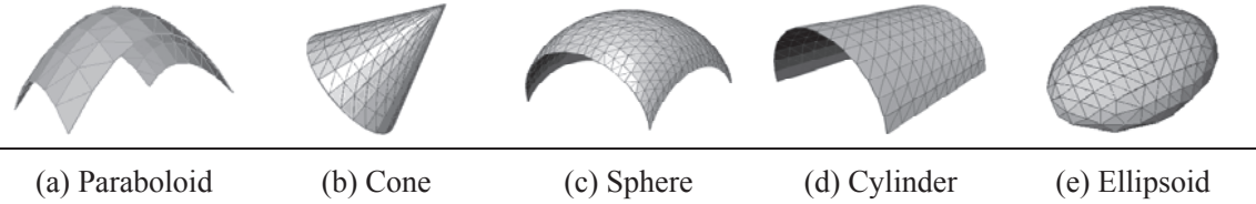
Figure 4-1: Types of systematic error of planar shapes
