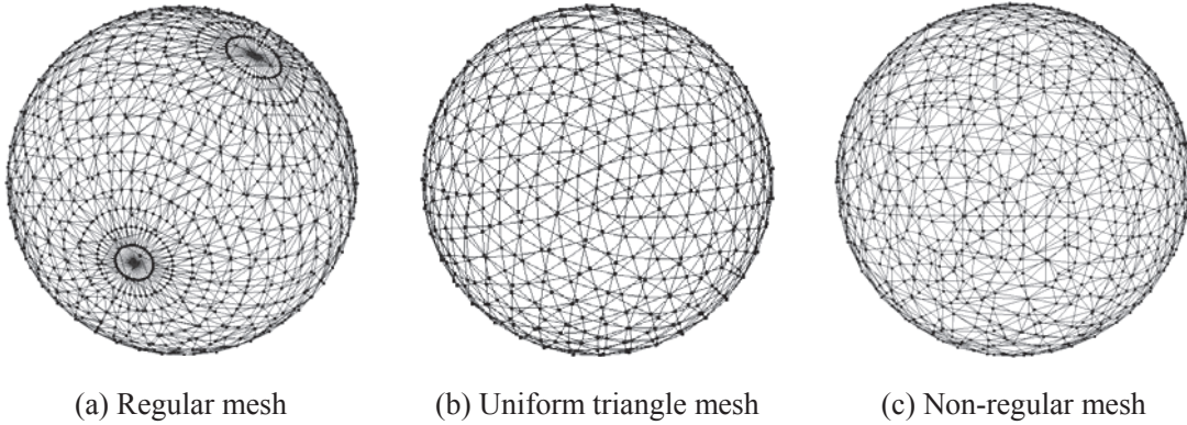
Figure 3-6: Mesh structure
