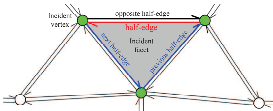
Figure 3-1: Half-edge data structure
