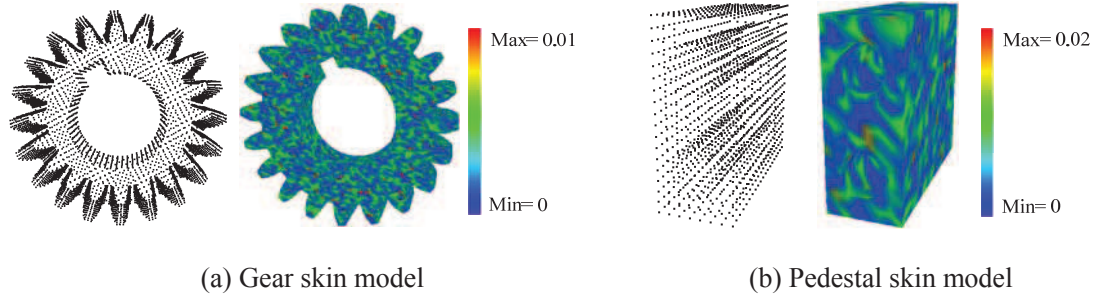
Figure 3-40: RGB visualization based on vertex normal
