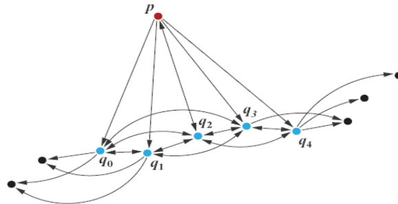
Figure 2-12: The Nearest-neighbor graph criterion
