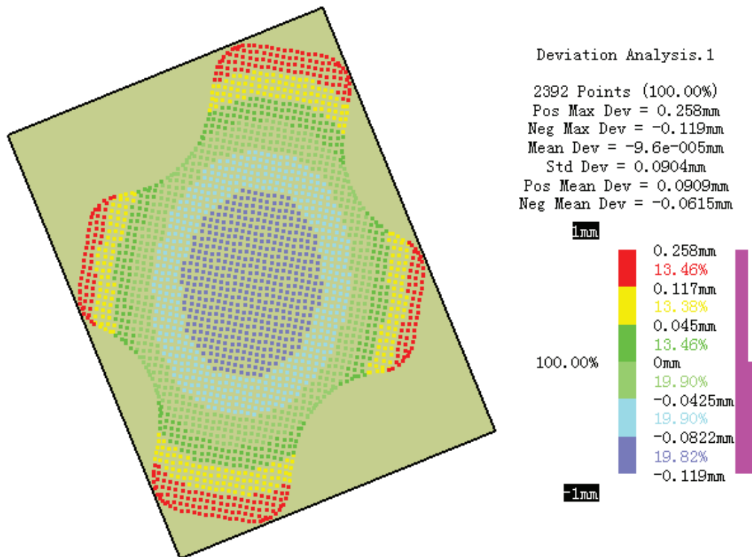
Figure 5-12: Analysis of skin model with systematic errors
