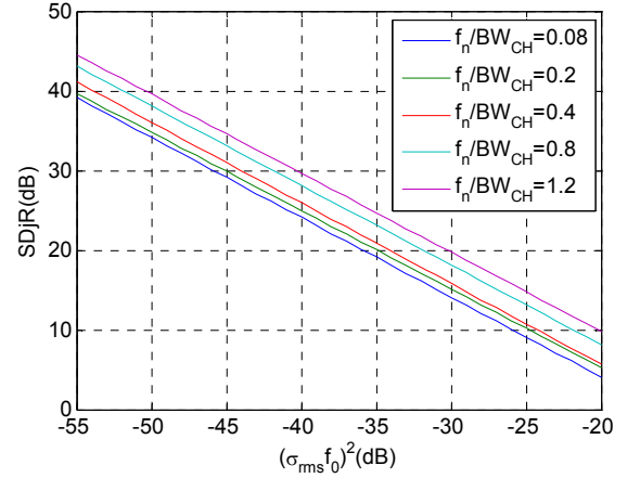
Figure 6-13 : SDjR \times (\sigma_{rms} f_0)^2 for different f_n / BW_{ch}
