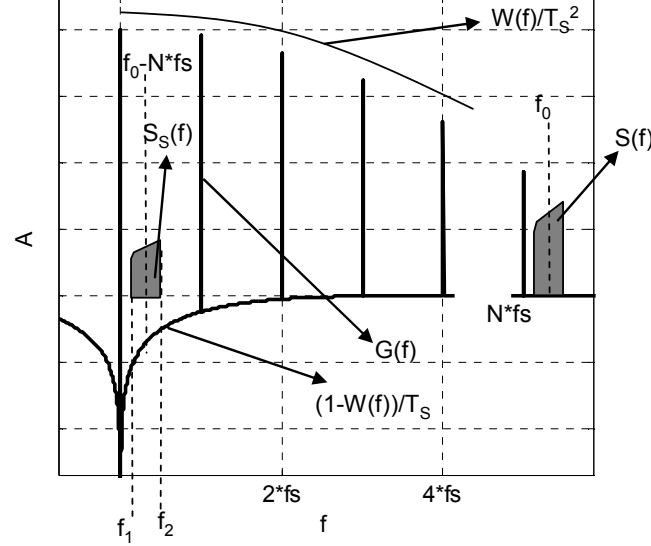
Figure 6-4 : Spectral representation of S(f) , the sampled spectrum S_s(f) and G(f) for jittered BPS
