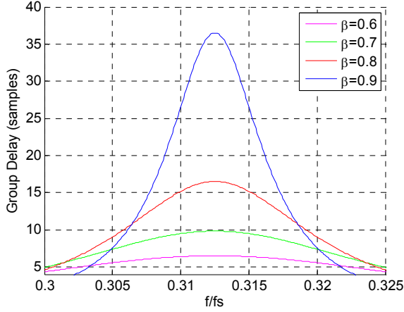
Figure 5-22 : Filter group delay for different \beta
