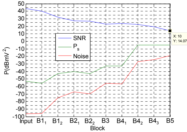
Figure 4-48 : Simulated SNR per block, BT-LE
