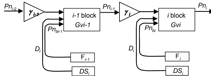
Figure 3-12 : System noise path block diagram with arbitrary additional source of distortion
