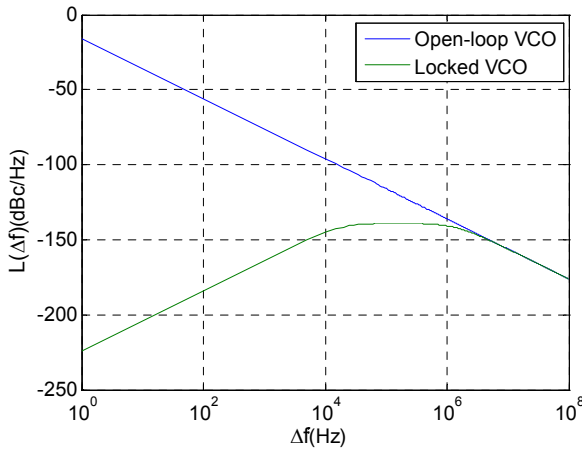
Figure 6-8 : The VCO phase noise
