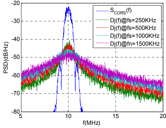
Figure 6-12 : S_{CORRS}(f) and Dj(f) @ f_s=100\text{MHz}
