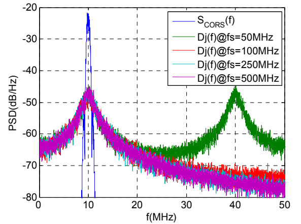
Figure 7 : S_{CORS}(f) and Dj(f)
