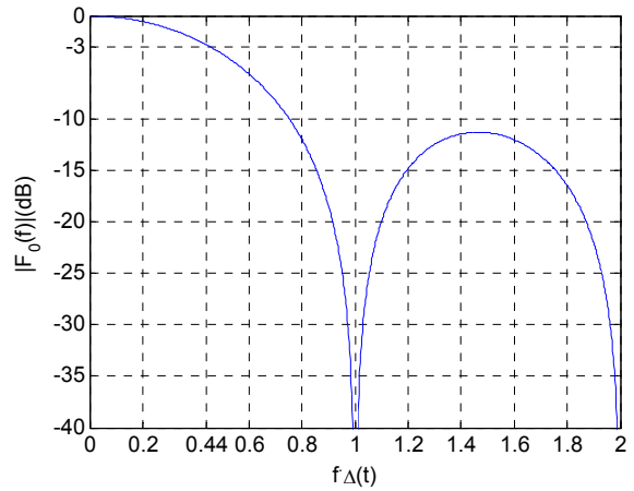
Figure 2-12 : The charge sampling sinc filter
