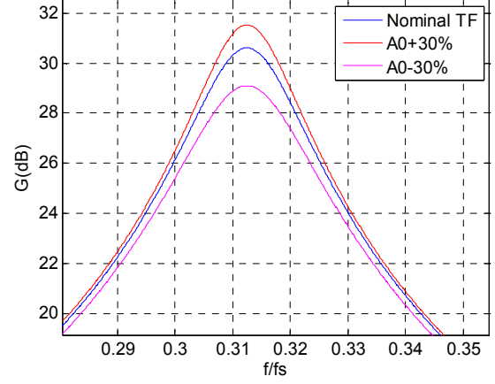
Figure 5-28 : IIR TF around the pole, A_0 = 100 .
