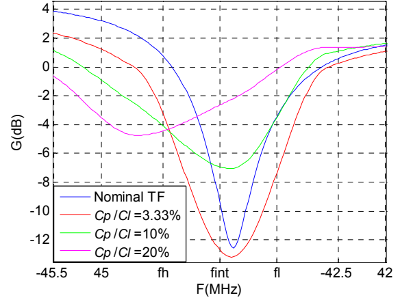
Figure 5-48 : Effect of the parasitic capacitances around the interferer @ -f_s/2 + f_s/16
