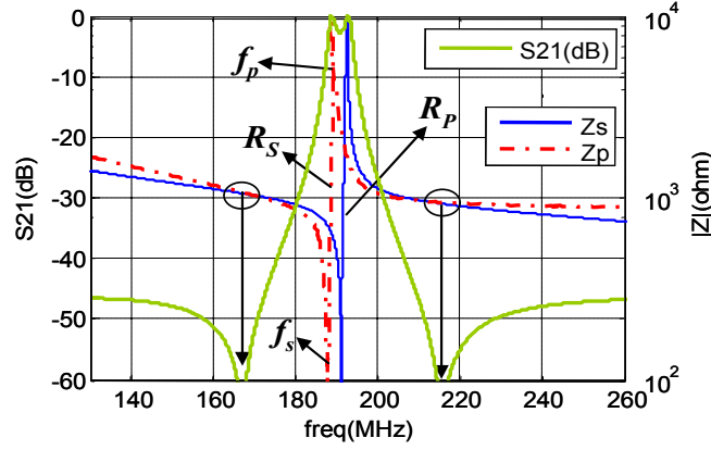
Figure 4-57 Lattice filter response and Z_{RS} and Z_{RP}
