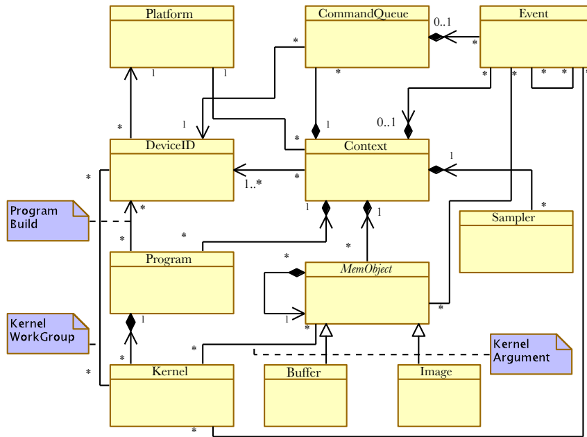
Figure A.6: OpenCL UML Class Diagram
