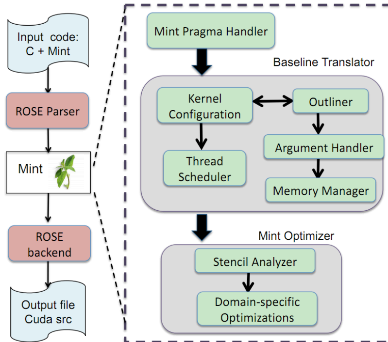
Figure 1.5: Modular design of Mint Translator and translation flow. Source: author's article [143]
