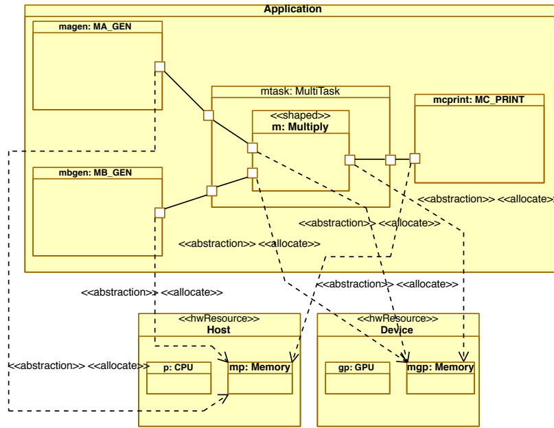
Figure 3.8: Data Allocation
