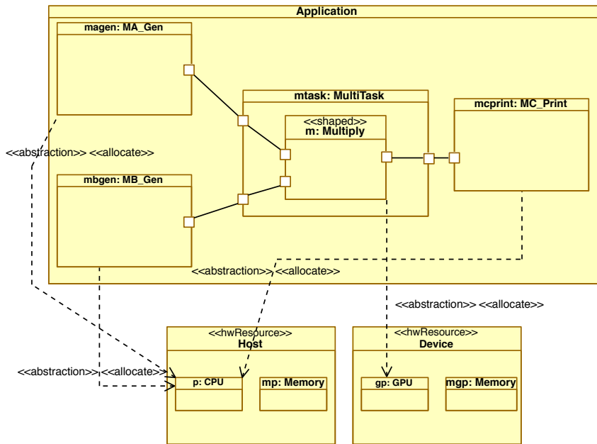
Figure 3.7: Task Allocation
