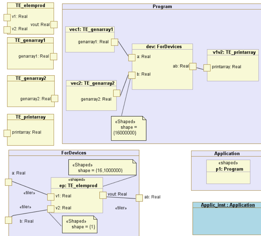
Figure 6.9: Vector Product Application Model
