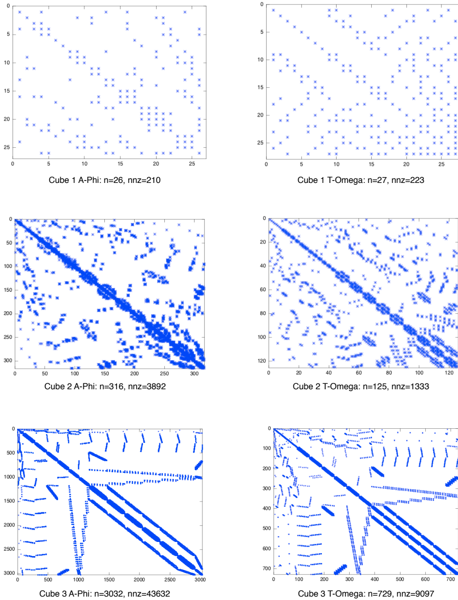
Figure 8.7: Cube 1 to 3: Sparse Matrices from Assembly Process
