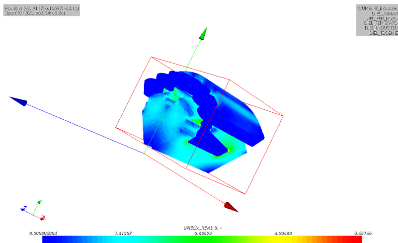
Figure 8.18: Post-processing results: \mathbf{B} field for the alternator example
