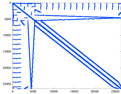
Cube 4 A-Phi: n=26416 , nnz=407176
