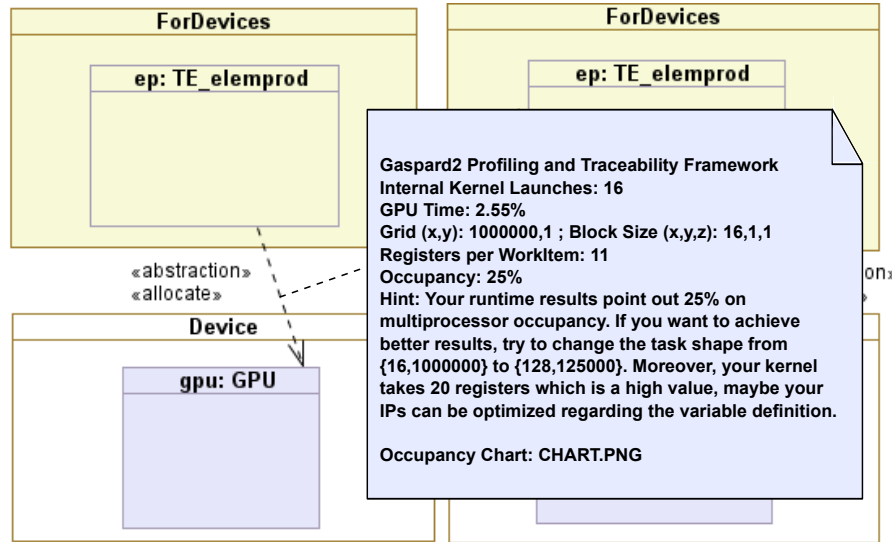
Figure 6.14: Annotated Model
