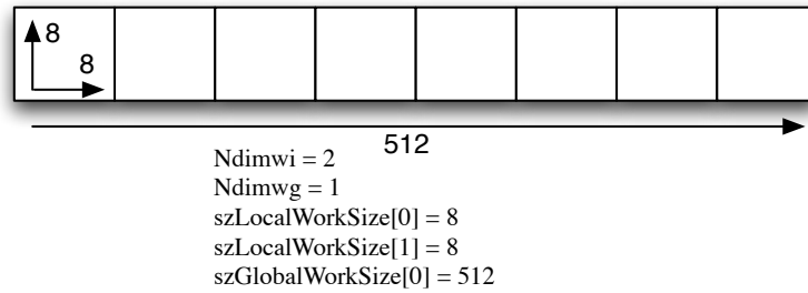
Figure 5.11: Grid Example
