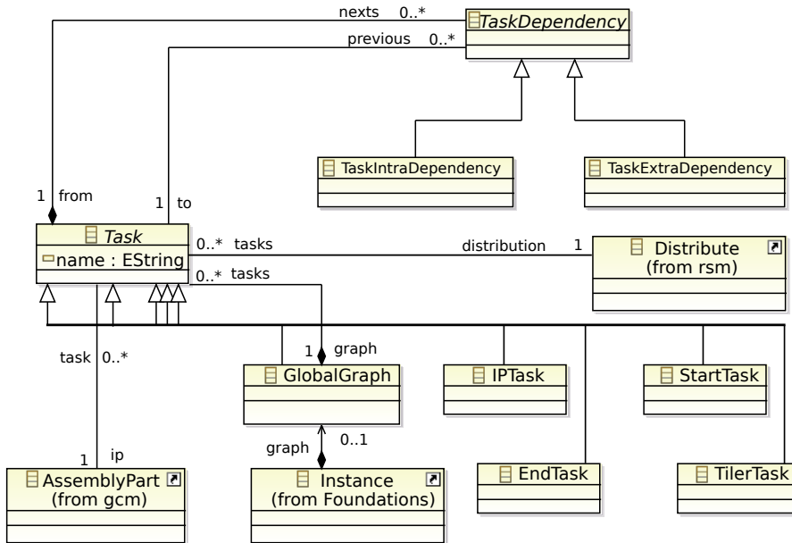
Figure 4.5: Global Task Graph Metamodel
