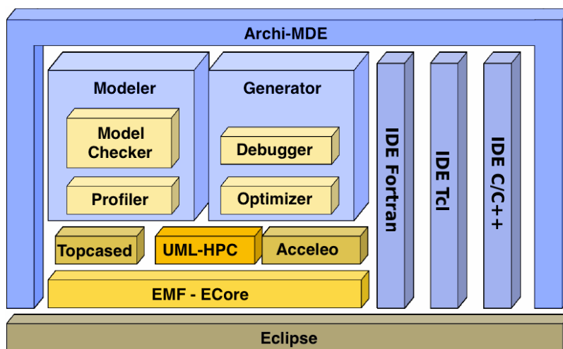
Figure 1.1: Architecture of the plug-in Archi-MDE. Source: author's article [98].
