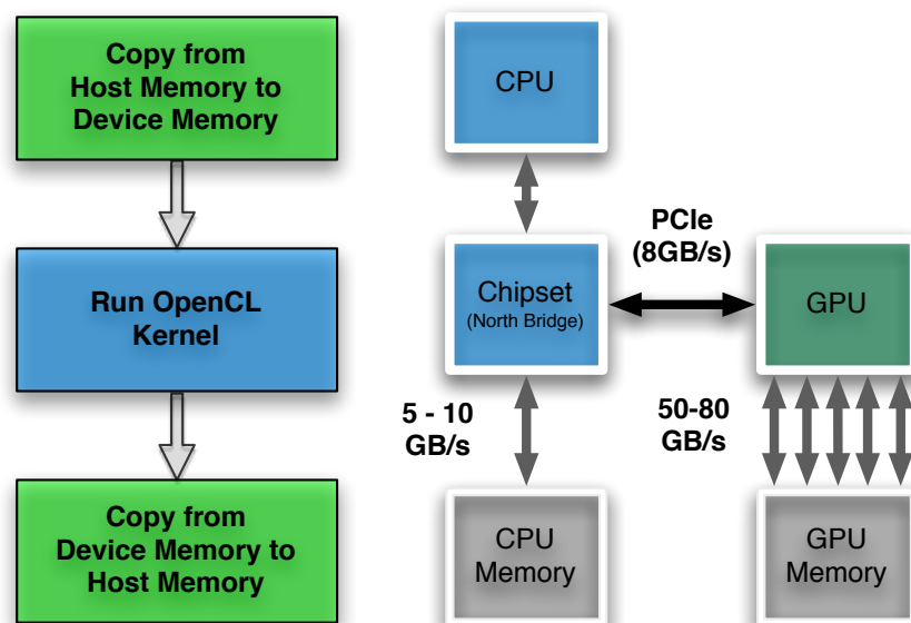
Figure 6.1: Typical Approach with Memory Copy
