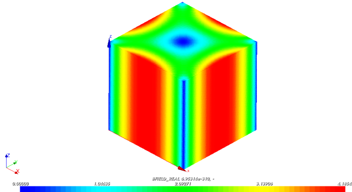
Figure 8.16: Post-processing results: \mathbf{B} field for the cube
