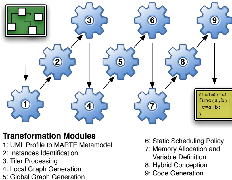
Figure 5.3: The UML/MARTE-to-OpenCL Transformation Chain
