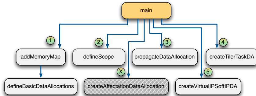
Figure 5.6: Memory Mapping Transformation Module Overview
