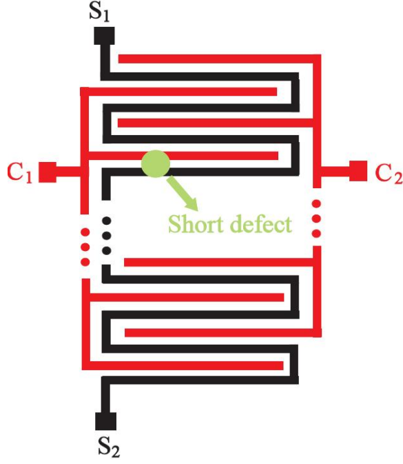
Figure 5.1: Comb-string-comb structure for defect resistance measurement [13].
