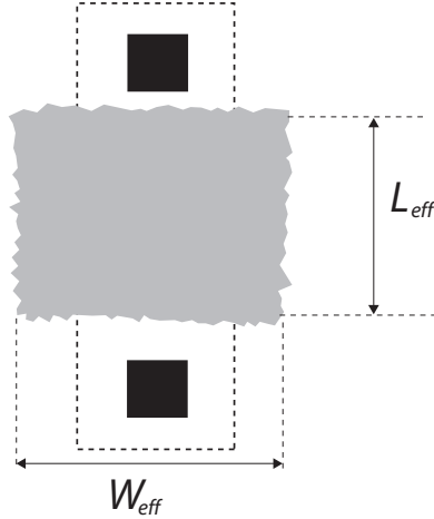
Figure 2.6: Local geometrical variations on L_{eff} and W_{eff} .
