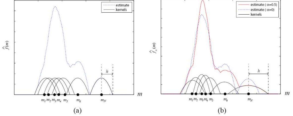
Figure 4.2: KDE method in the 1-dimensional case: (a) estimate in (4.1) where the same kernel is centered on each observation; (b) adaptive estimate in (4.3) where the bandwidth of the individual kernel varies.
