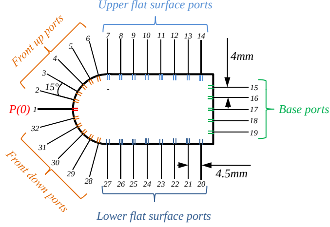
Figure 2.5: locations, grouping and numbering of the pressure ports on the main cylinder.
