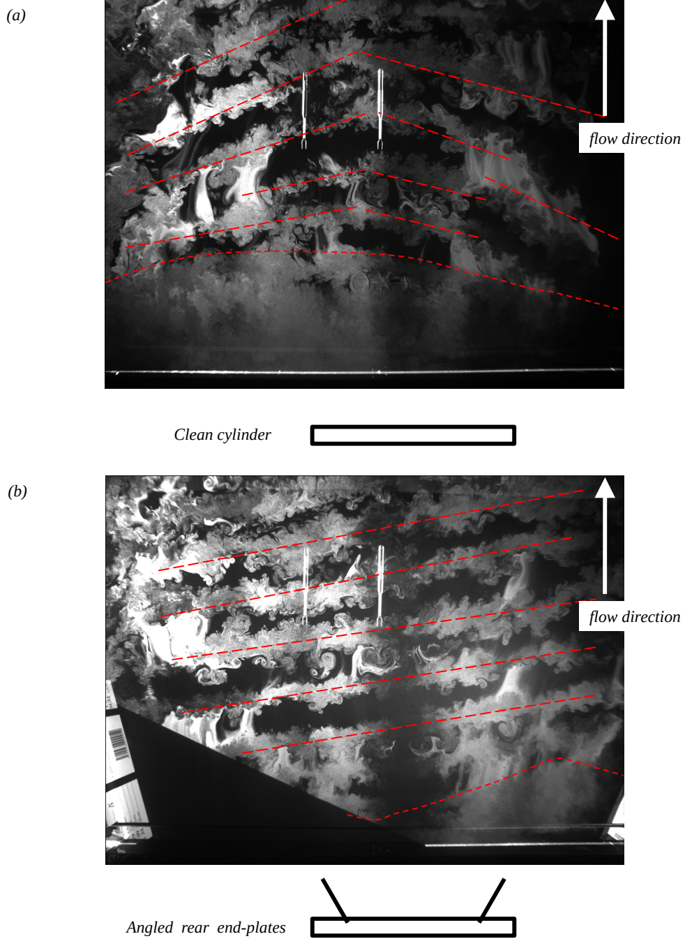
Figure C.3: Visualization of the turbulent wake with a d = 3mm control cylinder in IS configuration for (a) "clean" bluff cylinder and (b) bluff cylinder with rear end-plates at \alpha = \pm 30^\circ .
