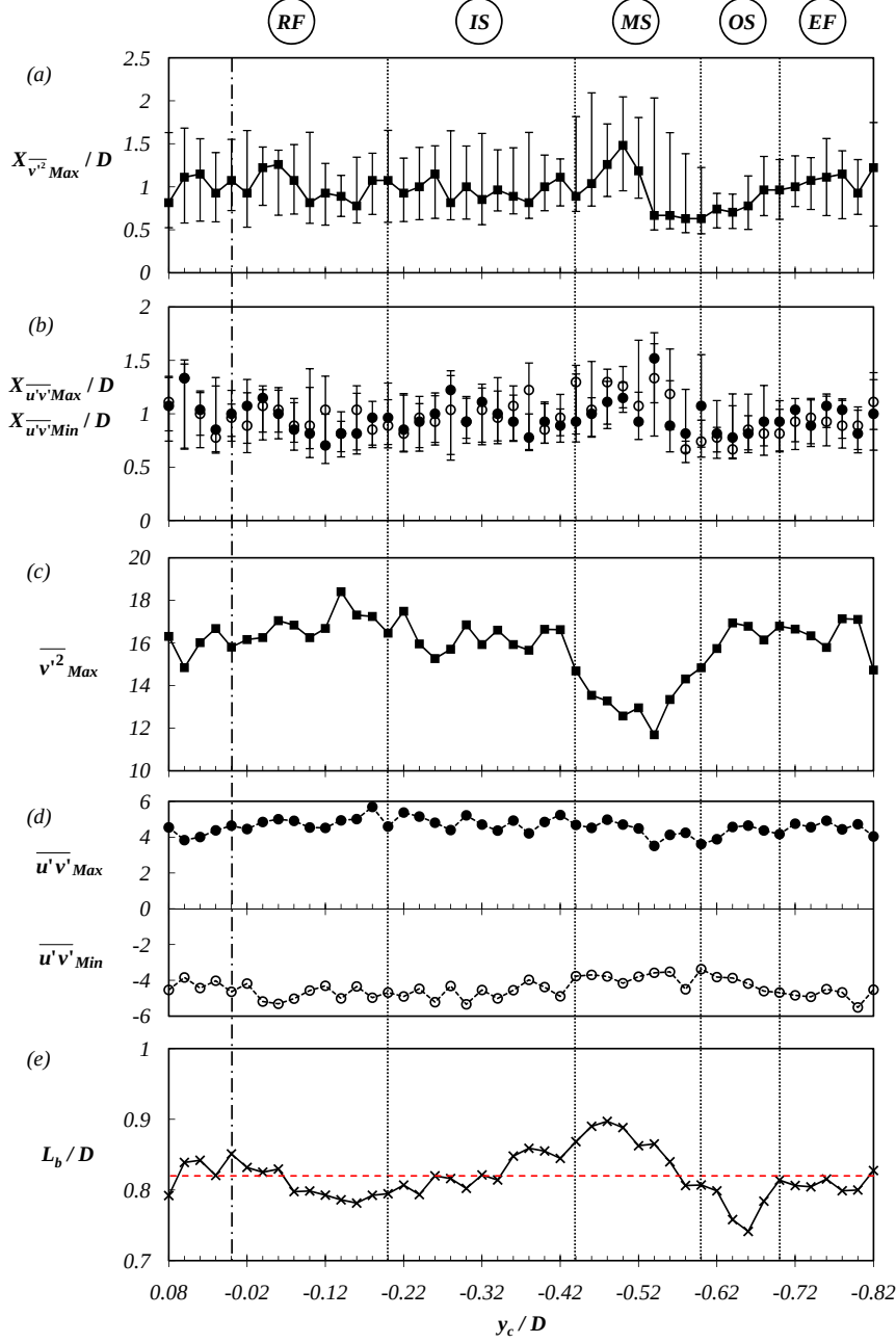
Figure 4.16: Amplitudes and streamwise locations of the extrema of Reynolds stress components \overline{v'^2}(x, y) and \overline{u'v'}(x, y) for positions of the 1mm control cylinder ( x_c/D = 0.4 , -0.82 < y_c/D < 0.08 ): (a) position of the maximum of \overline{v'^2} , (b) position of the maximum (filled circles) and the minimum (empty circles) of \overline{u'v'} , (c) amplitude of the maximum of \overline{v'^2} , (d) amplitudes of the maximum (filled circles) and the minimum (empty circles) of \overline{u'v'} and (e) size of the recirculation bubble L_b/D . Notation RF , IS , MS , OS and EF refers to configurations defined in section 4.2.2. Error bars denote the streamwise length of the first iso-line around the maximum (see figure 4.14).
